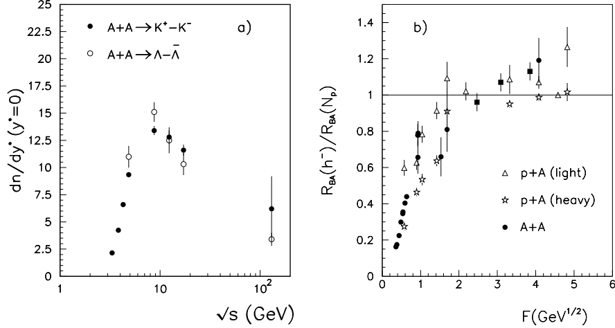
Figure 3. a) Energy dependence of \Lambda - \bar{\Lambda} and K^+ - K^- mid-rapidity multiplicities b) The ratio R_{BA}(h^-)/R_{BA}(N_p) for p+A and A+A reactions versus Fermi energy F (for the explanation see text)
