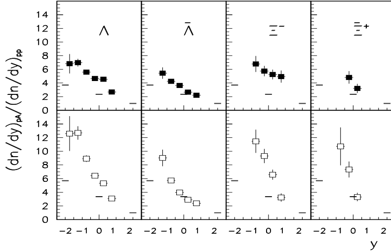
Figure 5. Ratios of hyperon multiplicities in centrality selected p+Pb and minimum bias p+p collisions. The experimental results for the first ( \langle\nu\rangle=3.7 ) and the second ( \langle\nu\rangle=5.7 ) centrality bin, are shown by full and open squares, respectively. The predictions of the WNM at backward, central and forward rapidities are indicated by the solid lines.
