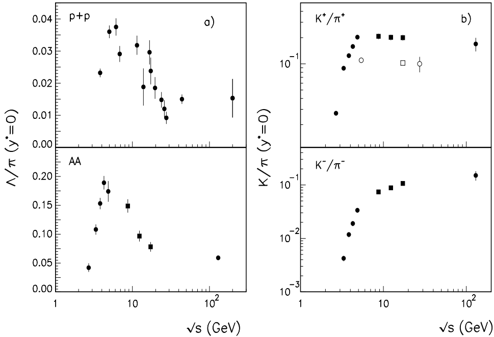
Figure 4. a) Energy dependence of \Lambda/\pi ratio at mid-rapidity in p+p (upper plot) and A+A (lower plot). b) Energy dependence of K^+/\pi^+ (upper plot) and K^-/\pi^- (lower plot) at mid-rapidity in A+A (full symbols) and p+A [9] (open symbols). Preliminary NA49 results are indicated by squares.
