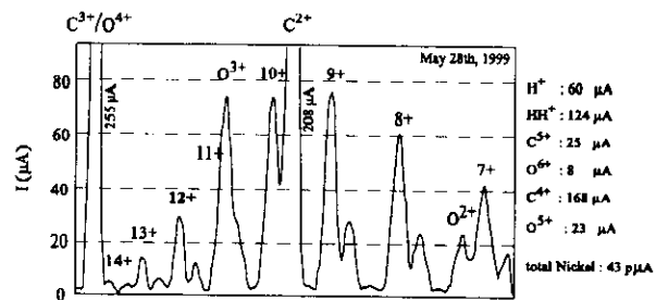
Figure 2. {}^{58}\text{Ni} spectrum, with 50 \mu\text{A} of \text{Ni}^{11+}
