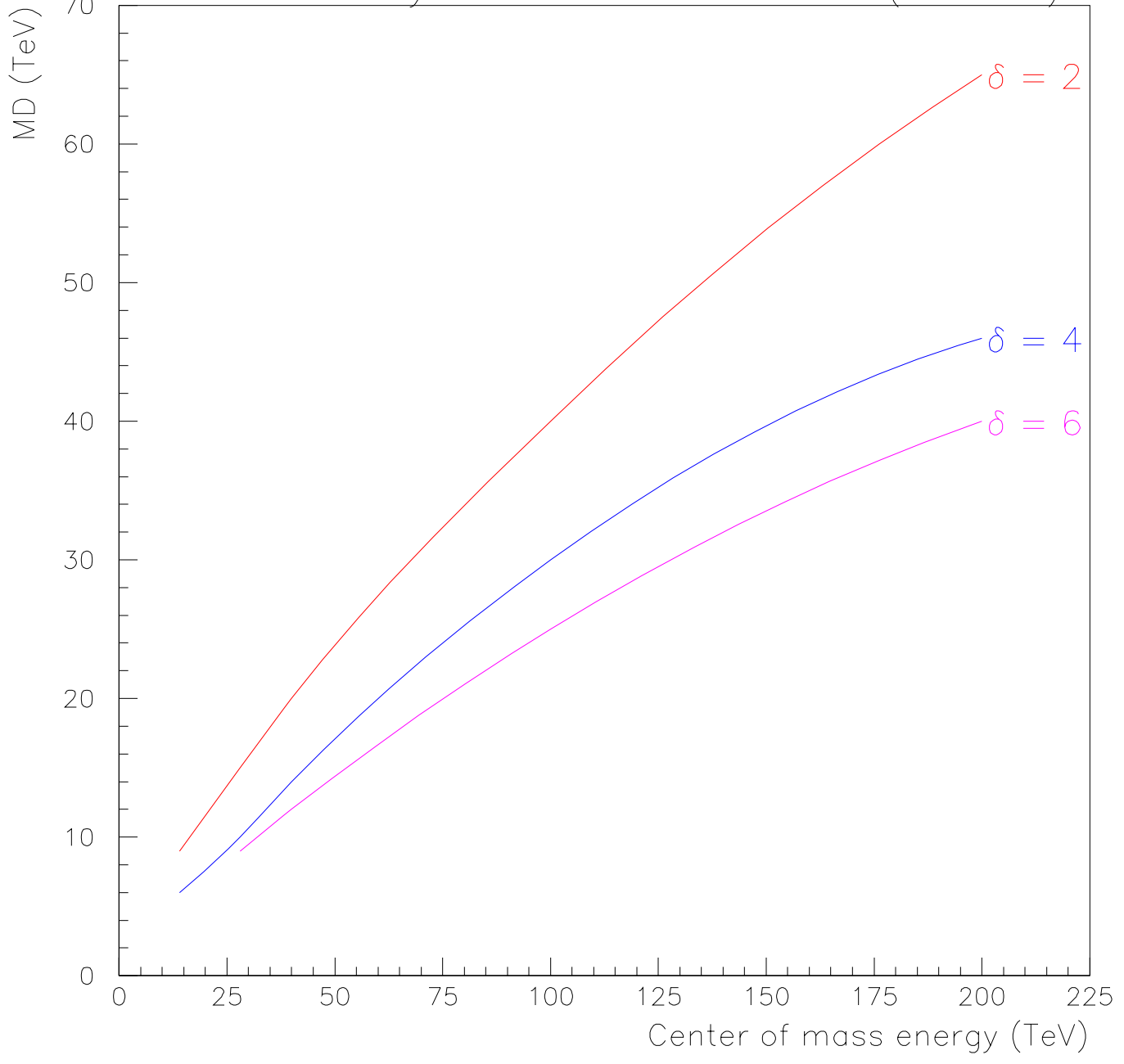
VLHC Sensitivity to ADD Extra Dimensions ( 100 \text{ fb}^{-1} )
