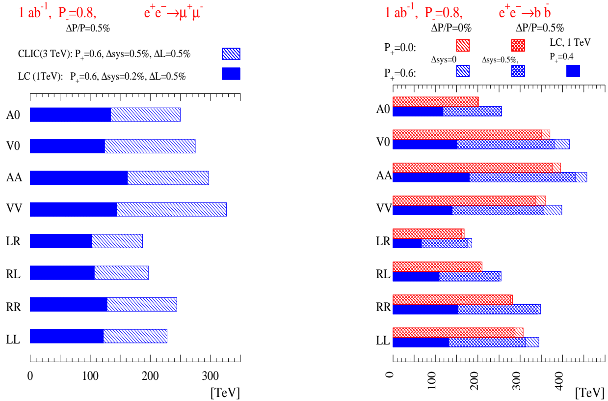
FIG. 2: Limits on the scale \Lambda of contact interactions in e^+e^- \rightarrow \mu^+\mu^- , b\bar{b} for CLIC operating at 3 TeV (dashed histogram) compared to a 1 TeV LC (filled histogram) for different models and the \mu^+\mu^- (left) and b\bar{b} (right) channels. The electron polarisations \mathcal{P}_- is taken to be 0.8 and the positron \mathcal{P}_+ to be 0.6. For comparison the upper bars in the right plot show the sensitivity achieved without positron polarisation. The influence of systematic uncertainties is also shown.
