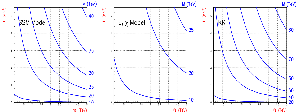
FIG. 1: The 95% C.L. sensitivity contours in the L vs. \sqrt{s} plane for different values of M_{Z'} in the SSM model (left) and in the E_6 \chi model (center) and for different values of the compactification scale M in a five dimensional extension of the SM with fermions on the boundary (right).
