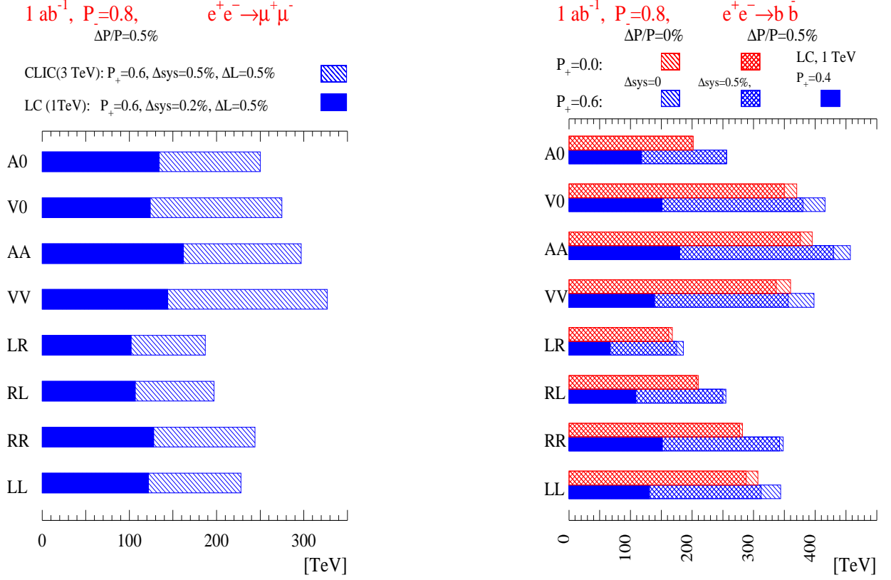
FIG. 2: Limits on the scale \Lambda of contact interactions in e^+e^- \rightarrow \mu^+\mu^- , b\bar{b} for CLIC operating at 3 TeV (dashed histogram) compared to a 1 TeV LC (filled histogram) for different models and the \mu^+\mu^- (left) and b\bar{b} (right) channels. The electron polarisations \mathcal{P}_- is taken to be 0.8 and the positron \mathcal{P}_+ to be 0.6. For comparison the upper bars in the right plot show the sensitivity achieved without positron polarisation. The influence of systematic uncertainties is also shown.
