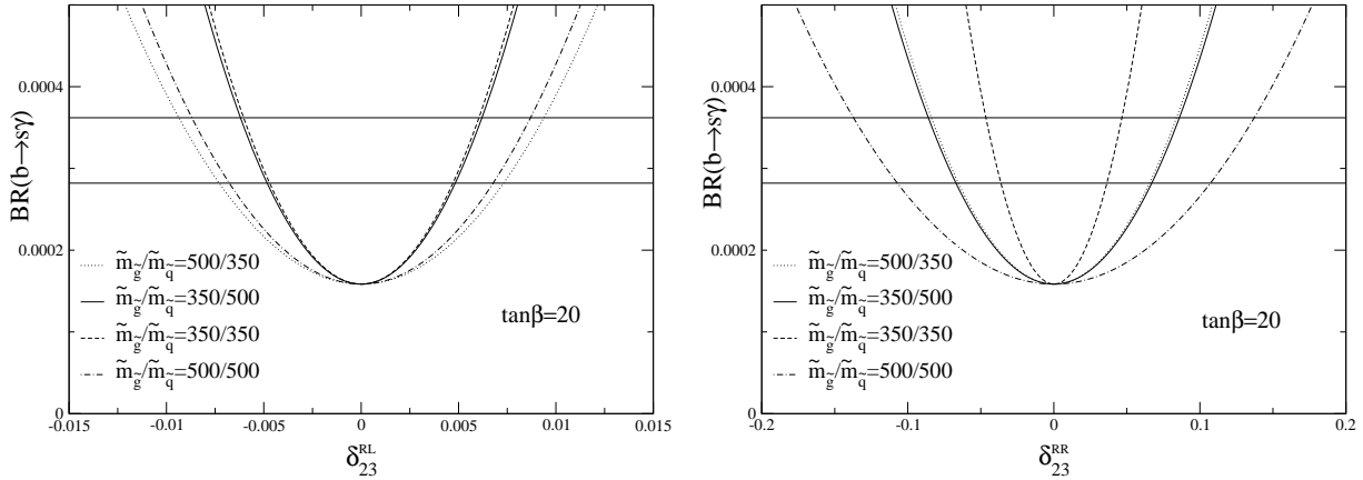
Figure 1: The dependence of b \rightarrow s \gamma branching ratio on \delta_{23}^{RL} and \delta_{23}^{RR} for different values of m_{\tilde{g}}=m_D , for \tan \beta = 20 and \mu = 350 GeV. All of the other off-diagonal entries except the one displayed in the axes, are assumed to vanish. C_{7,\beta}(W) = 0 is assumed. The horizontal lines represent the 1\sigma experimental allowed region.
