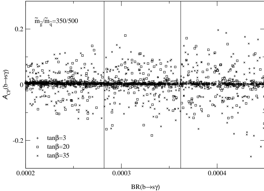
Figure 5: A symmetry vs branching ratio for three different values of \tan\beta , with m_{\tilde{g}}=m_{\tilde{q}}=350=500 , and M=350 GeV. All the off-diagonal entries except R_{23}^{RL} and R_{23}^{RR} are assumed to vanish. The vertical lines represent the 1 \sigma experimental allowed region.
