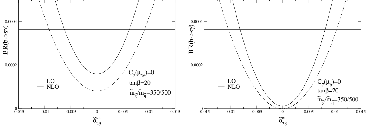
Figure 3: Dependence of b \rightarrow s branching ratio on \delta_{23}^{\text{RL}} for \tilde{m}_{\tilde{g}} = \tilde{m}_{\tilde{q}} = 350 = 500 , \tan \beta = 20 and \mu = 350 GeV. All the other off-diagonal entries, except the one displayed in the axes, are assumed to vanish. In the plots we show the result obtained using LO (dashed line) and NLO (full line) formula for the b \rightarrow s branching ratio, setting respectively C_{7,\beta}(\mu_W) = 0 (left plot) and C_{7,\beta}(\mu_b) = 0 (right plot). The horizontal lines represent the 1\sigma experimental allowed region.
