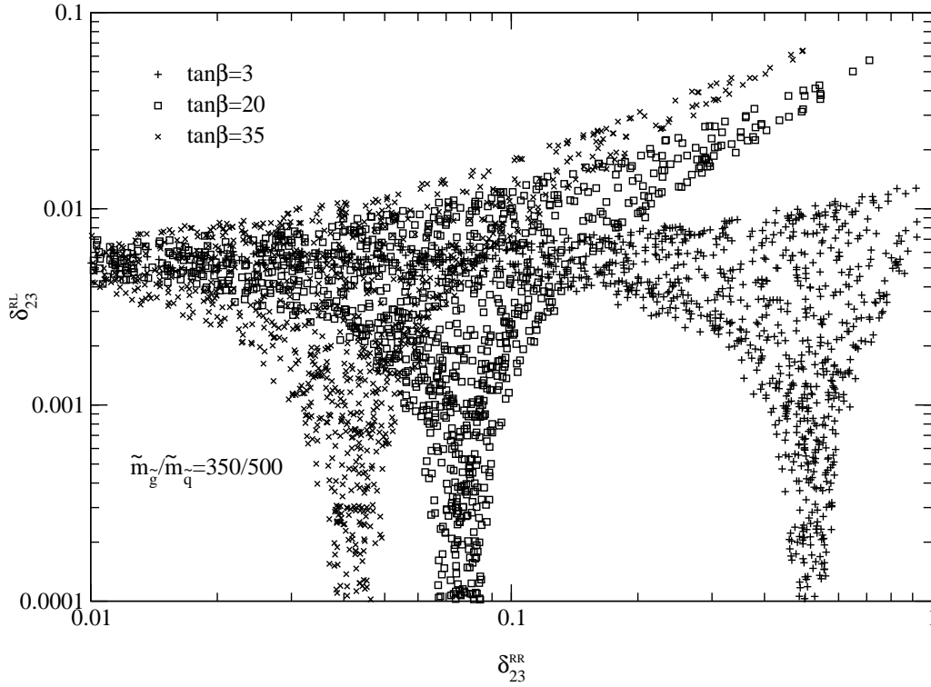
Figure 4: 1 -allowed region in the (\delta_{23}^{RR}, \delta_{23}^{RL}) parameter space for three different values of \tan \beta , with the other parameters fixed to m_g = m_q = 350=500 , and \mu = 350 GeV. All the other off-diagonal entries, except the one displayed in the axes, are assumed to vanish.
