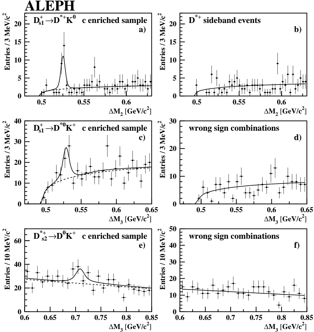
Figure 4: Reconstructed mass-difference distribution for the c -quark-enriched event sample. The full curve is the result of an unbinned log-likelihood fit and the dashed curve represents the combinatorial background.
