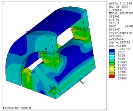
Figure 5: Sliding Shunt
