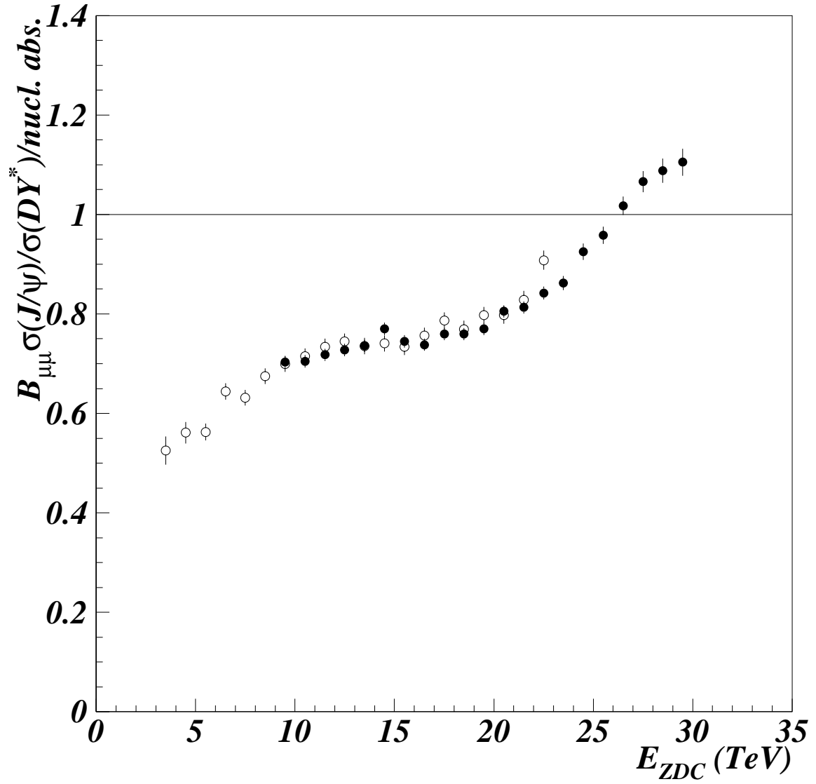
Figure 6: The \sigma_{J/\psi}/\sigma_{D^*} ratio divided by the absorption curve, as a function of E_{ZDC} . The full symbols refer to the 1996 data and the open symbols to the 1998 data.
