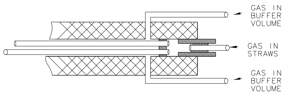
Figure 5.5: Scheme of parallel drift gas flows into the straw tubes and the surrounding buffer volume. Gas enters the straw tubes (shown at the left hand side) through a manifold.
