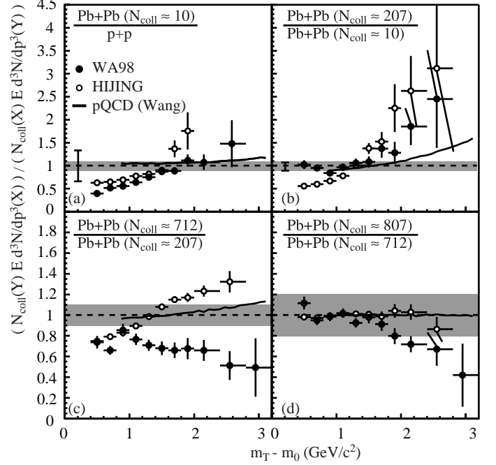
Fig. 14. Ratios of invariant multiplicity distributions of neutral pions normalized to the number of binary collisions. The upper left plot (a) shows the ratio of peripheral Pb+Pb collisions to the parameterization of p+p [3]. The other plots (b-d) show different ratios of a more central sample to a more peripheral sample of Pb+Pb collisions. The filled circles show the experimental results, the open circles are results from the HIJING event generator and the solid lines similar ratios from pQCD calculations including p_T broadening [42]. The grey bands show the estimate of the systematic error due to the systematic error in the \pi^0 distribution. The additional error bar in (a) and (b) shows the normalization uncertainty due to the calculation of the number of collisions and the absolute cross section normalization relative to p+p.
