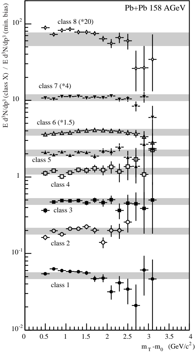
Fig. 8. Ratios of invariant multiplicities of neutral pions for Pb + Pb collisions of different centralities to minimum bias distributions as a function of m_T - m_0 , with class 1 being the most peripheral and class 8 the most central sample. The grey bands show the estimate of the centrality dependent systematic error.
