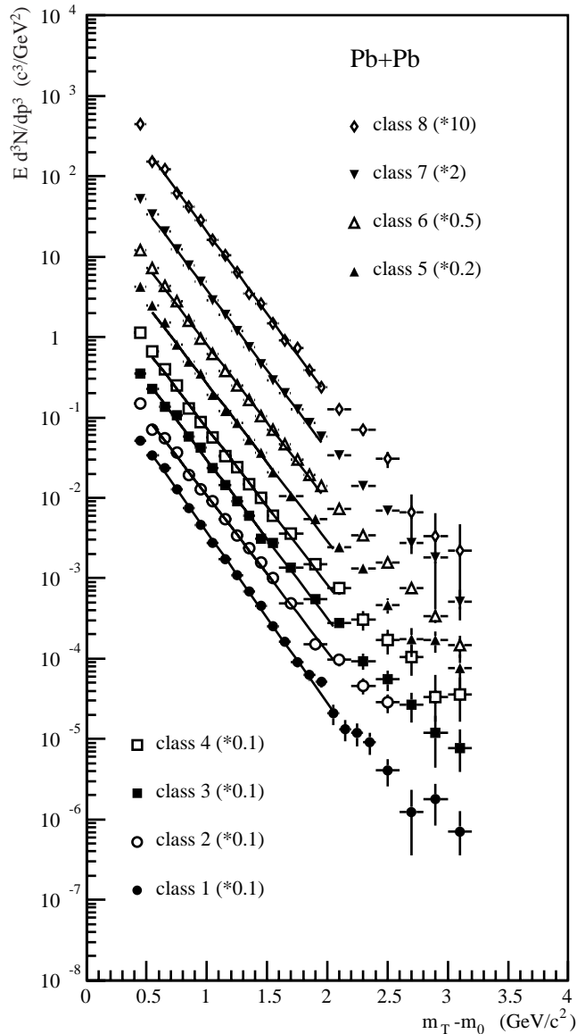
Fig. 7. Invariant multiplicities of neutral pions for Pb + Pb collisions of different centralities as a function of m_T - m_0 . The solid lines show exponential fits to the spectra.
