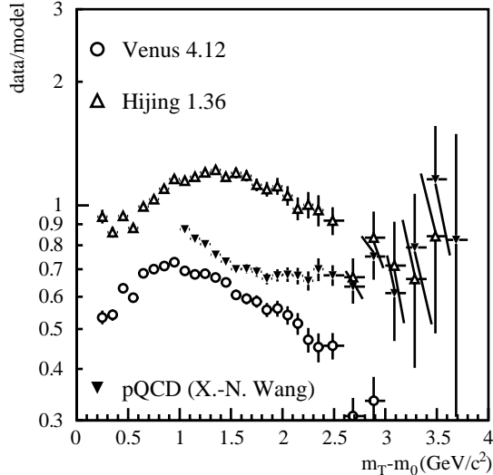
Fig. 6. Ratios of measured invariant multiplicities of neutral pions to those from Monte Carlo event generators for central Pb + Pb collisions as a function of m_T - m_0 .
