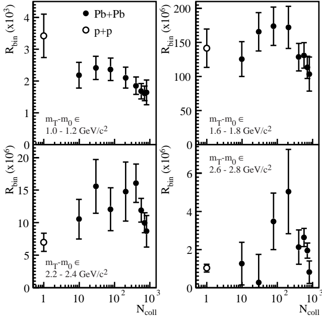
Fig. 15. Multiplicities of neutral pions normalized to the number of binary collisions R_{bin} = (E d^3N/dp^3)/N_{coll} as a function of N_{coll} for different ranges of transverse mass as indicated in the pictures. The filled circles show the experimental results for Pb+Pb reactions, the open circles the parameterization for p+p reactions (Eq. 3). The error bars contain statistical and systematic errors added in quadrature.
