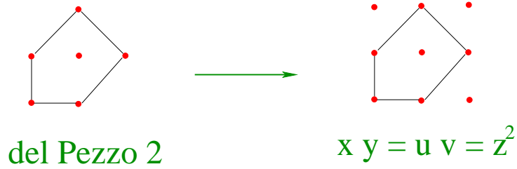
Figure 9: Embedding the toric diagram of dP_2 into the orbifolded conifold described as xy = uv , uv = z^2 .
