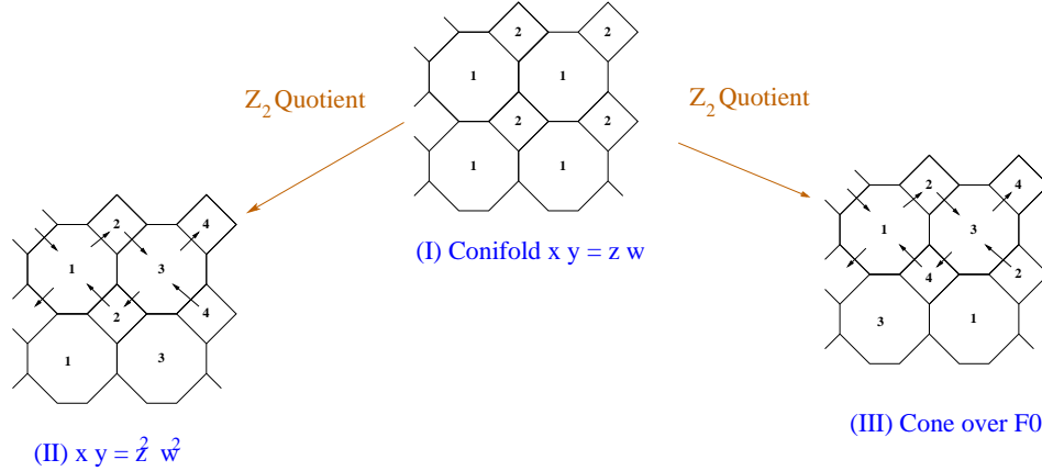
Figure 7: (I) Brane diagram for the conifold. Identifications in the infinite periodic array of boxes leads to a two-dimensional unit cell, whose sides are identified in the obvious manner. From (I) we have 2 types of \mathbb{Z}_2 quotients: (II) Brane diagram for the \mathbb{Z}_2 quotient of the conifold xy = z^2 w^2 , which is a case of the so-called generalised conifold. The identifications of sides are trivial, not tilting. The final spectrum is the familiar non-chiral spectrum for a brane interval with two NS and two NS' branes (in the alternate configuration); (III) Brane diagram for the \mathbb{Z}_2 quotient of the conifold yielding the complex cone over F_0 . The identifications of sides are shifted, a fact related to the specific 'tilted' refinement of the toric lattice.
