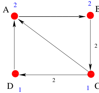
Figure 14: A non-Abelian phase of the complex cone over dP_3 . This example is Picard-Lefschetz dual to the other 4 examples in Figure 12 but not Seiberg dual thereto.
