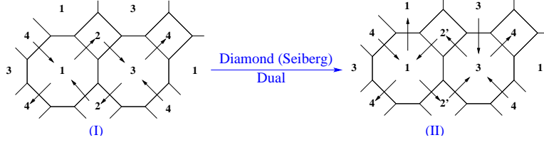
Figure 6: Seiberg duality from the brane diamond construction for the generalized conifold xy = z^2 w^2 . Part (I) corresponds to the brane interval picture with alternating ordering of NS- and NS 0 -branes, whereas part (II) matches the other ordering.
