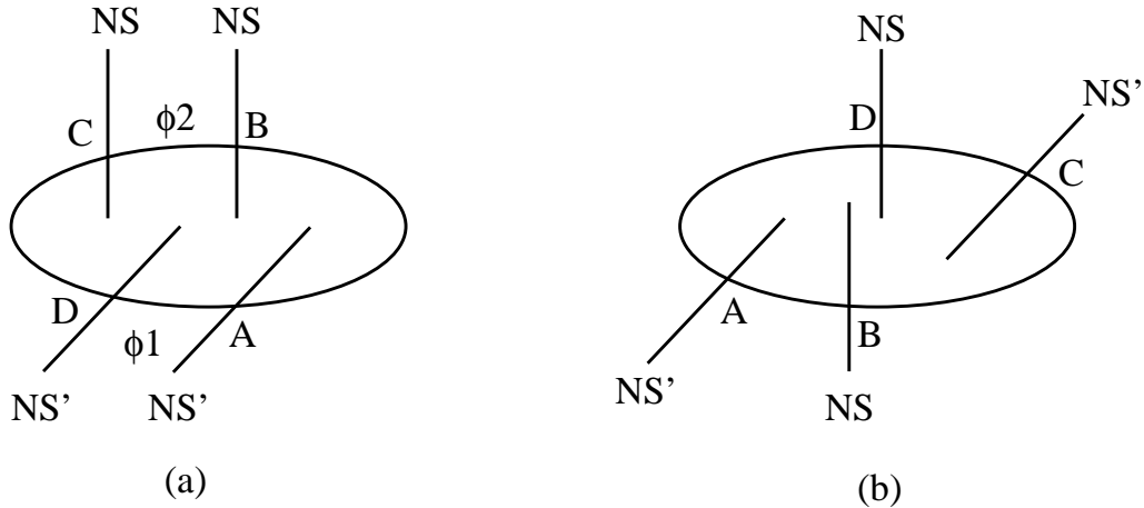
Figure 1: The two possible brane setups for the generalized conifold xy = z^2w^2 . They are related to each other passing one NS-brane through an NS'-brane. A_i; B_i; C_i; D_i i=1,2 are bifundamentals while \phi_1; \phi_2 are two adjoint fields.
