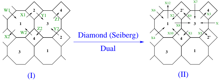
Figure 8: Brane diagram for the two cases of the cone over F_0 . (I) is as in Figure 7 and (II) is the result after the diamond duality. The resulting spectrum and interactions are those of the toric dual (and also Seiberg dual) of the initial theory (I).
