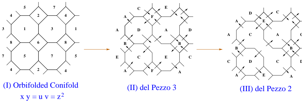
Figure 10: (I) Brane diagram for a \mathbb{Z}_2 \times \mathbb{Z}_2 orbifold of the conifold, namely xy = z^2; uv = z^2 . From this we can partially resolve to (II) the cone over dP_3 and thenceforth again to (III) the cone over dP_2 , which we shall discuss in the context of Seiberg duality.
