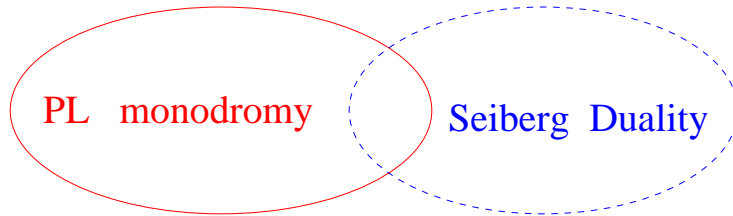
Figure 13: The relation between Picard-Lefschetz monodromy and Seiberg Duality. For certain classes of the theories they coincide while in general we can find examples of each which are not in the other.
