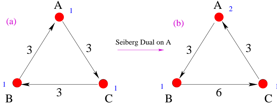
Figure 14: Seiberg Dualisation on node A of the \mathbb{C}^3/\mathbb{Z}_3 orbifold theory. The subsequent theory cannot be obtained by a Picard-Lefschetz monodromy transformation.
