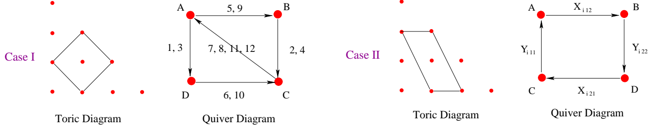
Figure 4: The quiver and toric diagrams of the 2 torically dual theories corresponding to the cone over the zeroth Hirzebruch surface F_0 .
