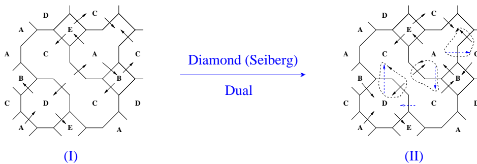
Figure 11: The brane diamond setup for the Seiberg dual configurations of the cone over dP_2 . (I) is as in Figure 10 and (II) is the results after Seiberg (diamond) duality and gives the spectrum for the toric dual theory. The added meson fields are drawn in dashed blue lines. Notice that applying the diamond dual rules carelessly one gets some additional vectorlike pairs, shown in the picture within dotted lines. Such multiplets presumably get massive in the Seiberg dualization, hence we do not consider them in the quiver.
