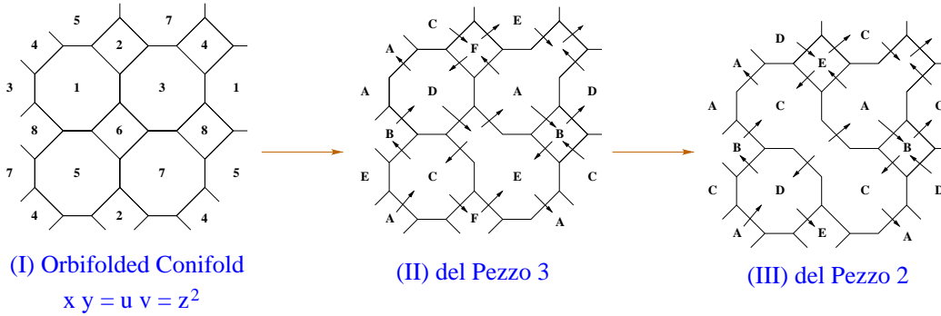
Figure 10: (I) Brane diamond for a \mathbb{Z}_2 \times \mathbb{Z}_2 orbifold of the conifold, namely xy = z^2; uv = z^2 . From this we can partial resolve to (II) the cone over dP_3 and thenceforth again to (III) the cone over dP_2 , which we shall discuss in the context of Seiberg duality.
