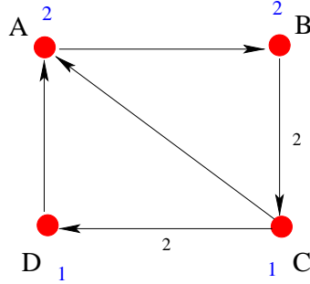
Figure 15: A non-Abelian phase of the complex cone over dP_3 . This example is Picard-Lefschetz dual to the other 4 examples in Figure 12 but not Seiberg dual thereto.
