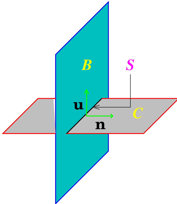
Figure 1: The brane-world B is perpendicular to the normal vector n . The four dimensional hypersurface C is orthogonal to the velocity vector u . The surface S = C \cap B is a set of comoving observers following matter on the brane. Note that the perturbed brane is not necessarily located at y = \text{constant} . The different metrics in the text are as follows: g_{ab} is the full ve{dimensional metric, h_{ab} is the induced metric on the brane B , u_{ab} is the induced metric on C and n_{ab} is the induced metric on the comoving hypersurface S .
