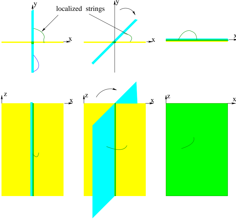
Figure 2: Rotating two branes from orthogonal position \theta = \pi/2 to parallel one \theta = 0 .
