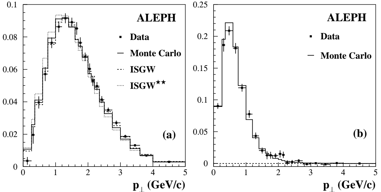
Figure 7: Comparison between the lepton p_{\perp} spectra measured in the data with the charge correlation analysis and that expected from simulation. (a) b \rightarrow X\ell\nu ; data are compared with the simulation corrected as described in Section 6.15, ISGW and ISGW** models. (b) b \rightarrow c \rightarrow X\ell\nu . All the spectra are normalized to unit area.
