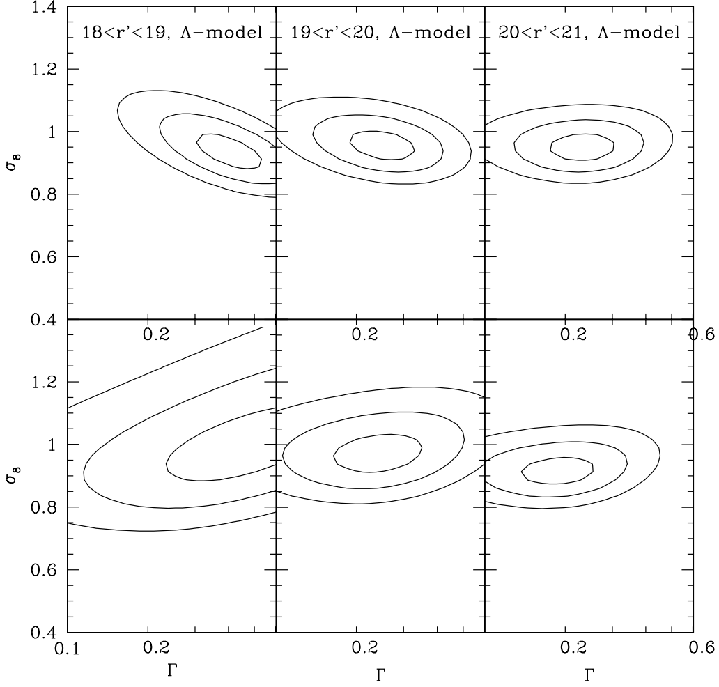
Fig. 7.— Likelihood contours (plotted at 1, 2, \text{ and } 3\sigma ) for \sigma_{8L} and the shape parameter \Gamma for three magnitude bins as indicated in the panels. These assume an \Omega_m = 0.3, \Omega_\Lambda = 0.7 cosmology. The redshift distribution dn/dz \propto z^2 e^{-(z/z_0)^{1.5}} with median redshifts z_m = 0.17, 0.24, 0.33 is used for the three panels respectively ( z_m = 1.412z_0 ). The KL expansion was truncated at 300 modes in the upper three panels. To ensure that only the linear modes are used, in the lower panels the expansion was truncated at 60, 150 and 250 modes (from left to right). The panel in the lower right is our best fit.
