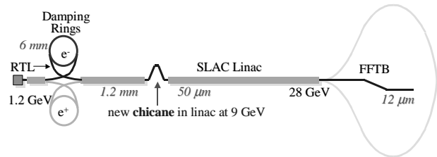
Figure 1. Layout of SLAC linac with 30-kA compression.
