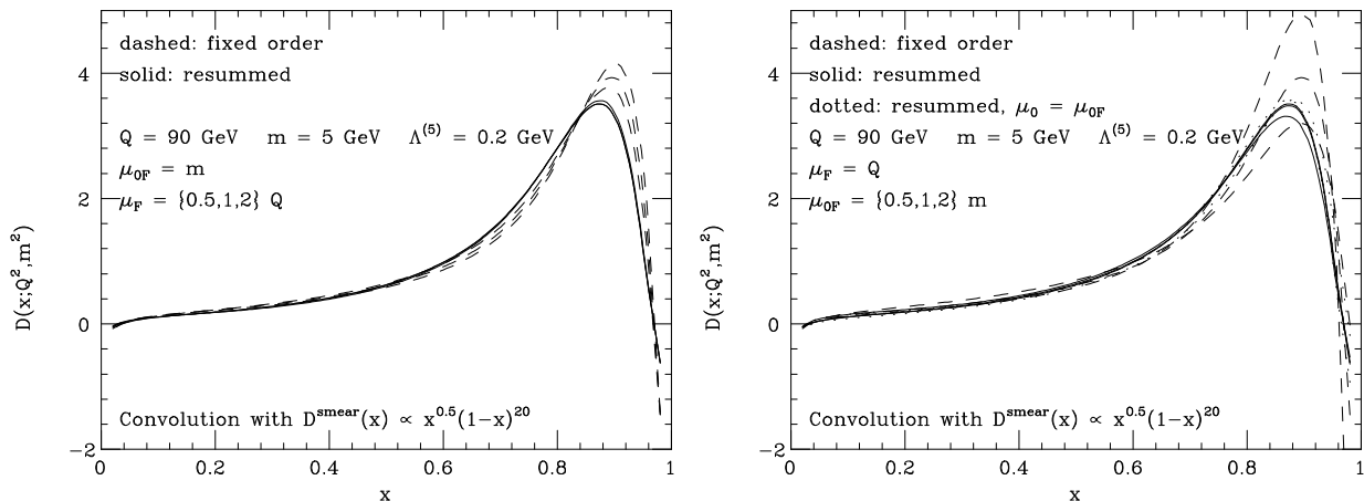
Figure 9: Dependence of the heavy-quark distribution \mathcal{D}(x) on the variations of the factorization scales \mu_F (left) and \mu_{0F} (right). Convolution with a smearing function D^{\text{smear}}(x) \propto x^{0.5}(1-x)^{20} , normalized to have D_{N=1}^{\text{smear}} = 1 , has been included for better visibility. The dotted lines in the right-hand plot are obtained by varying also the renormalization scale \mu_0 ( \mu_0 = \mu_{0F} = \{0.5, 2\} ).
