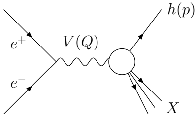
Figure 1: Inclusive production of a hadron h with momentum p in e^+e^- annihilation.
