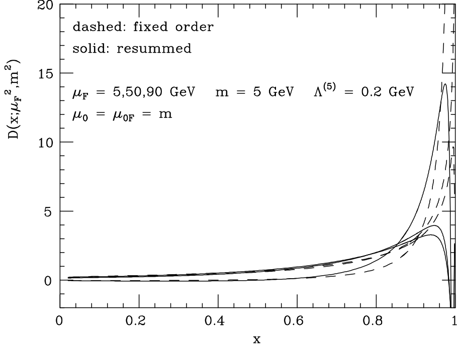
Figure 6: Effect of Sudakov resummation for the initial condition of the heavy-quark fragmentation function, evolved up to three different scales \mu_F = 5, 50, 90 GeV.
