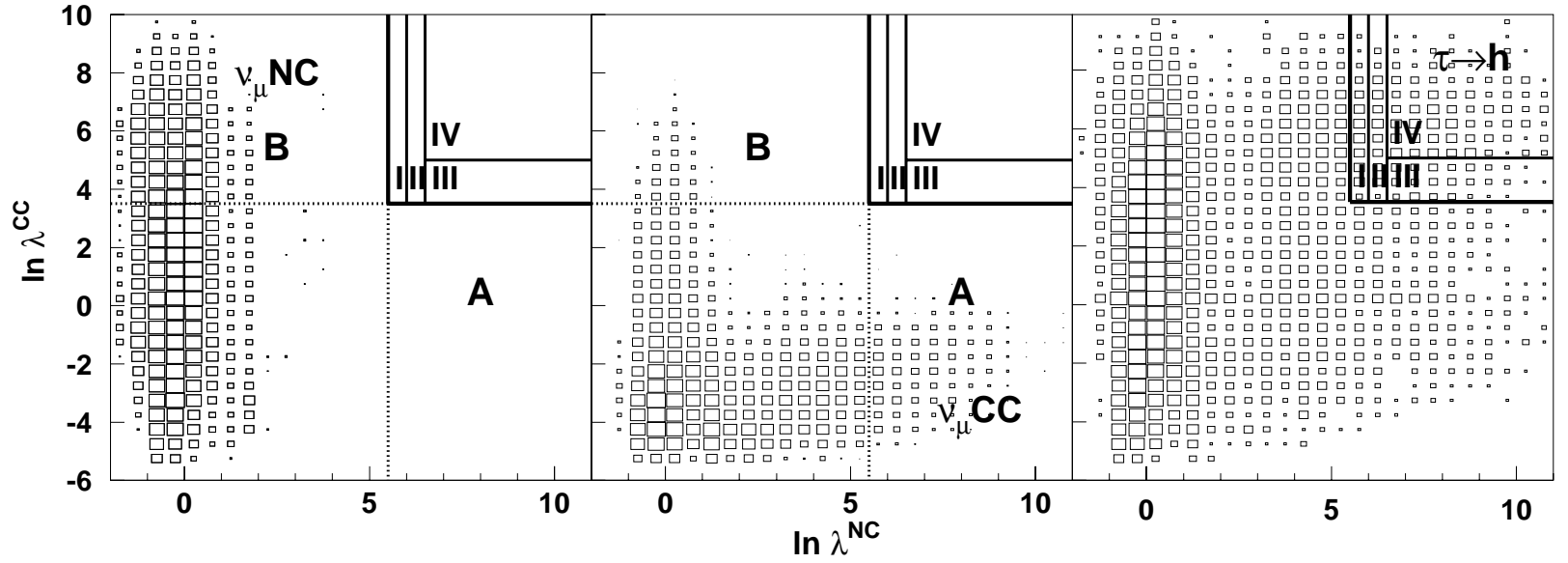
Fig. 7. Scatter plot of \ln \lambda^{\text{CC}} vs \ln \lambda^{\text{NC}} for MC backgrounds from \nu_\mu NC (left plot) and \nu_\mu CC interactions passing the first level veto (middle plot) and simulated \tau \rightarrow \nu_\tau \pi ( 0\gamma ) decays (right plot). The local bin densities are shown in logarithmic scale. The large box at the upper right corner, divided into four bins, defines the signal region, whereas the dotted lines show the control regions used to estimate the systematic uncertainties on CC (region A) and NC (region B) events.
