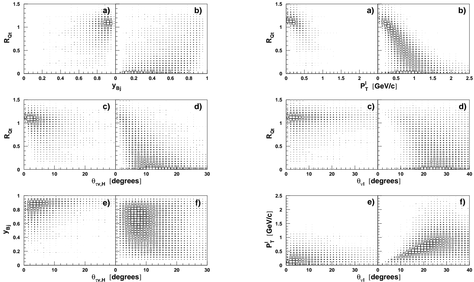
Fig. 3. Left plots: correlations between kinematic variables, not related to the internal \tau_V structure, used to construct \ln\lambda^S for wrong (a,c,e) and correct (b,d,f) combinations of \tau decay products in \nu_\tau\pi decays (Section 5.1). Right plots: correlations between kinematic variables used to construct \ln\lambda^V for wrong tracks (a,c,e) and for the true leading muon (b,d,f) in \nu_\mu CC events passing the first level veto (Section 5.3).
