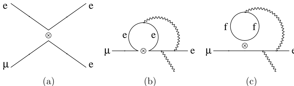
Figure 4: (a) Lepton flavor-violating four-fermion operator; (b) Example of a contribution to \mu \rightarrow e\gamma for f = e or \mu ; (c) Example of other fermions' contribution.
