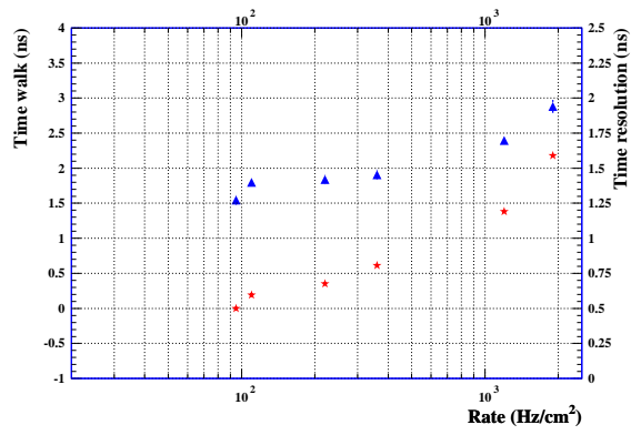
Fig. 6. Time walk (stars) and time resolution (triangles) as a function of the rate.
