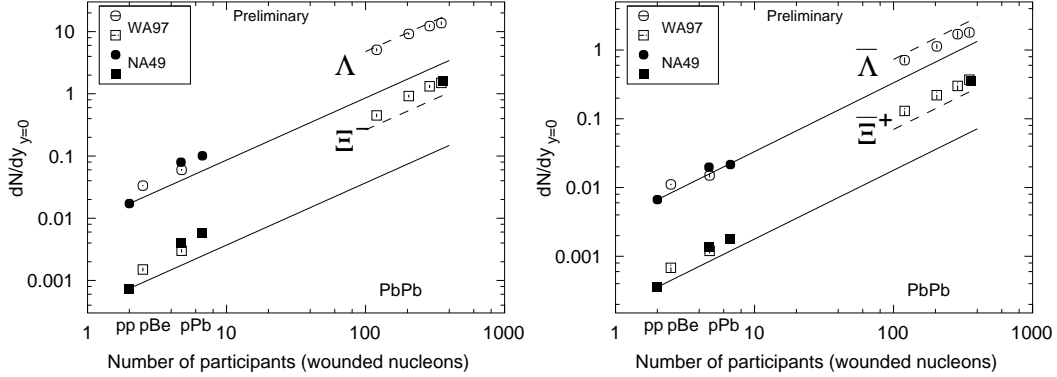
Figure 4: Midrapidity yields of hyperons in p+p, p+A and A+A collisions as a function of N_{part}
