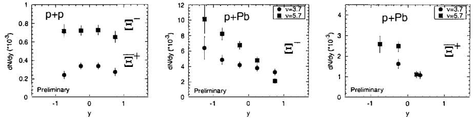
Figure 3: Cascade baryon yields in p+p (left) and in centrality controlled p+Pb collisions (middle and right)
