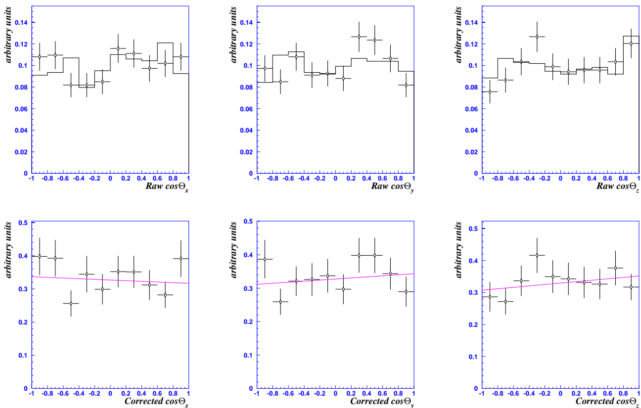
Figure 4: Top: normalized angular distributions ( \cos\theta_i ) for \bar{\Lambda} hyperons in reconstructed Monte Carlo events (histogram) and in data (points with error bars). Bottom: experimental angular distributions corrected for detector acceptance and selection effects; the polarization is given by the slope of the corresponding linear fit.
