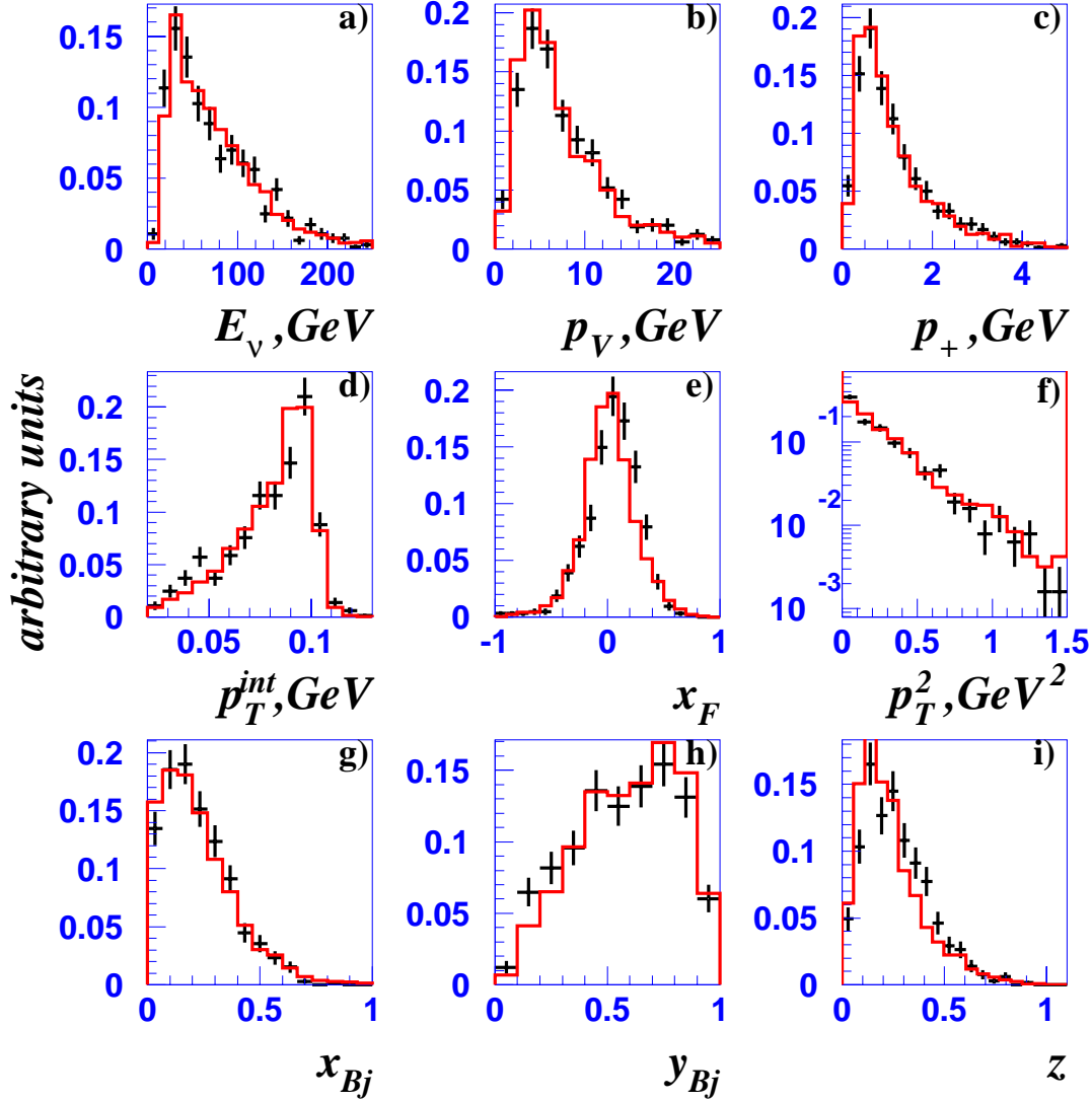
Figure 3: Comparison of reconstructed kinematic variables for \nu_\mu CC events containing identified \bar{\Lambda} hyperons for simulated (histogram) and data (points with error bars) events: a) neutrino energy, b) \bar{\Lambda} momentum, c) momentum of the outgoing \pi^+ from the \bar{\Lambda} decay, d) transverse component of the momentum of one of the outgoing charged tracks with respect to the V^0 direction (internal p_T ), e) x -Feynman, f) square of the transverse component of the \bar{\Lambda} momentum with respect to the hadronic jet direction, g) x -Bjorken, h) y -Bjorken, i) fraction of the total hadronic energy carried by the \bar{\Lambda} in the laboratory system.
