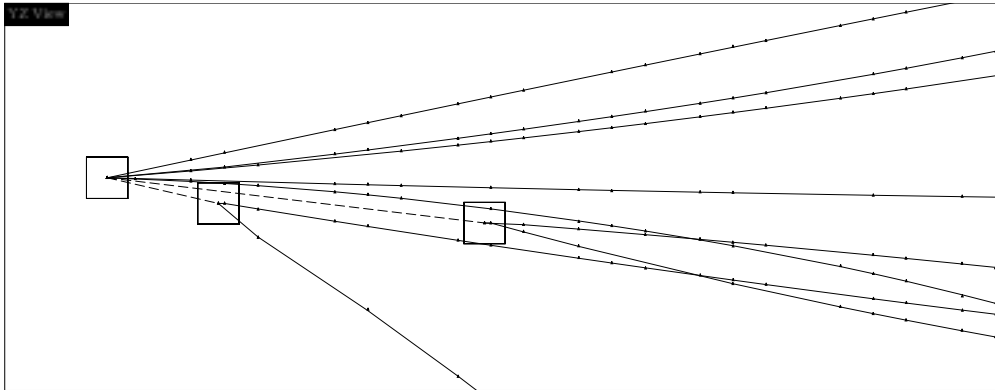
Figure 1: A reconstructed data event containing 2 V^0 vertices identified as \Lambda and \bar{\Lambda} decays by our identification procedure. The scale on this plot is given by the size of the vertex boxes ( 3 \times 3 \text{ cm}^2 ).
