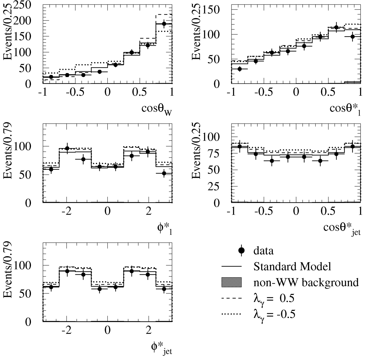
Figure 5: The distributions of the kinematic quantities \cos\theta_W , \cos\theta_l^* , \phi_l^* , \cos\theta_{jet}^* and \phi_{jet}^* from the combined sample of the evq\bar{q} and \mu\nu q\bar{q} channels at 189 GeV. The measured variables are the angle \theta_W between the W^- and initial e^- in the W^+W^- rest frame, the polar and azimuthal angles of the lepton, \theta_l^* and \phi_l^* , in the rest frame of its parent W , and the polar and azimuthal angles of a quark jet, \theta_{jet}^* and \phi_{jet}^* , in the rest frame of its parent W . As no quark flavour tagging is performed each of the two ambiguous solutions enters with a weight of 0.5. The data are represented by solid dots, while the solid and dashed histograms show distributions for Standard Model and non-standard values of \lambda_\gamma = \pm 0.5 .
