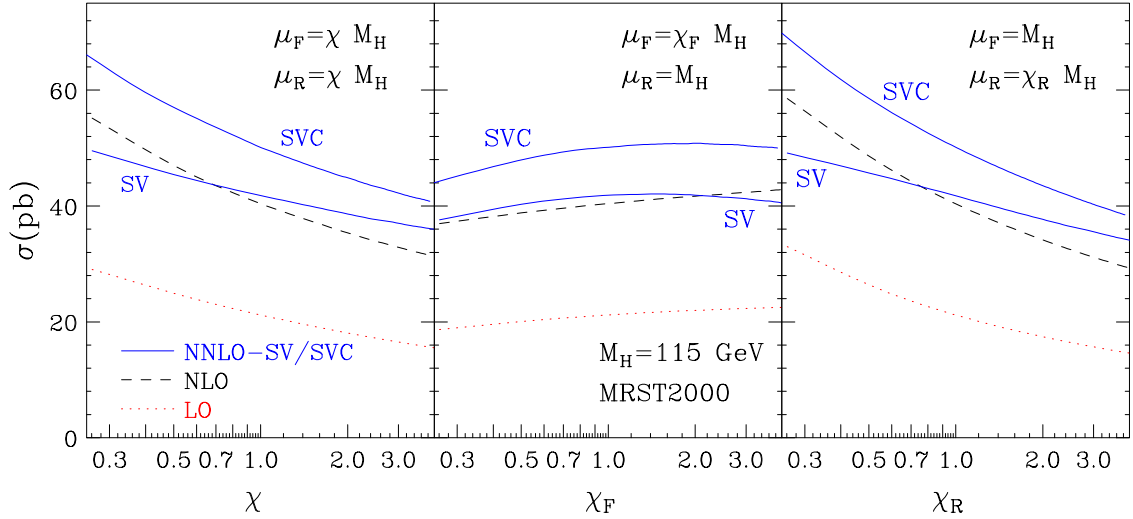
Figure 1: Scale dependence of the Higgs production cross section for M_H = 115 GeV at LO, NLO, NNLO-SV and NNLO-SVC.
