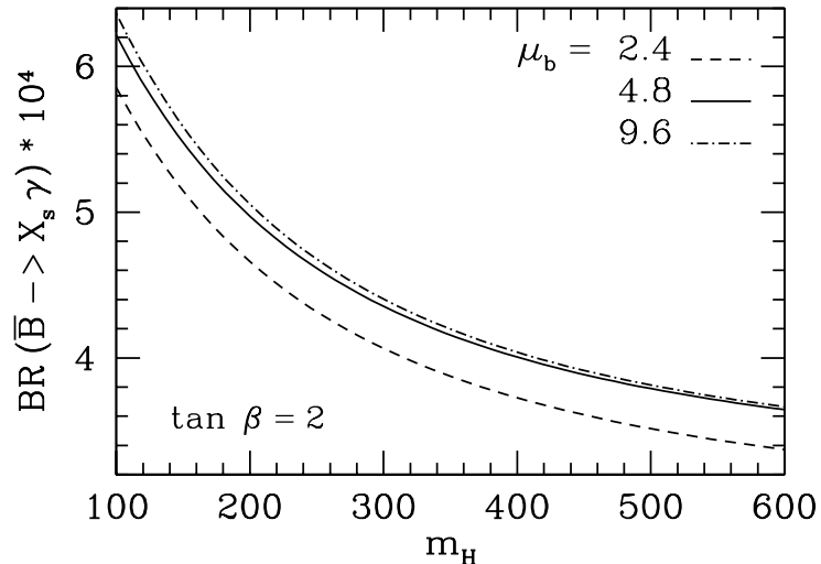
Figure 3: The branching ratio for B \rightarrow X_s \gamma as a function of the charged Higgs mass; figure taken from [29].
