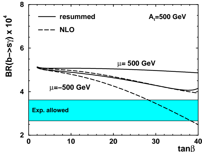
Figure 5: The rate for B \rightarrow X_s \gamma versus \tan \beta ; for the values of the parameters see text. Figure taken from [33].
