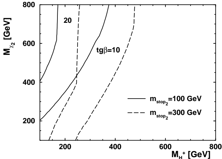
Figure 6: Allowed range in the M_{H^+}-M_{\tilde{\chi}_2^0} plane for different values of \tan \beta for two values of m_{\tilde{t}_2} . Figure taken from [33].
