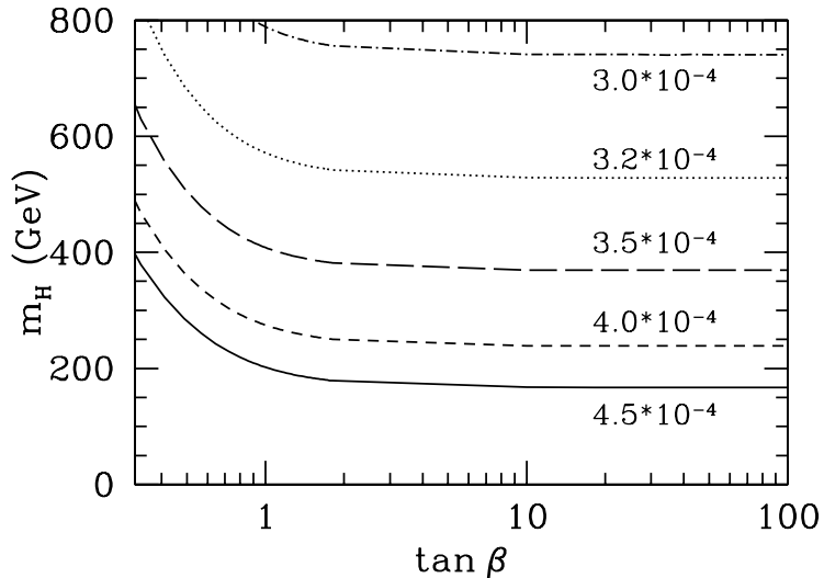
Figure 4: The \tan\beta - M_{H^+} plane; contours indicate different experimental values for B \rightarrow X_s\gamma ; figure taken from [29].
