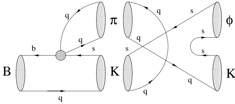
Figure 2: Rescattering processes contributing to B \rightarrow \phi K through annihilation topologies. The shaded circle represents insertions of current–current operators ( q \in \{u, d\} ).
