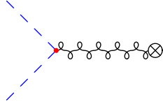
Figure 3: A diagram of order \tau^1 .
