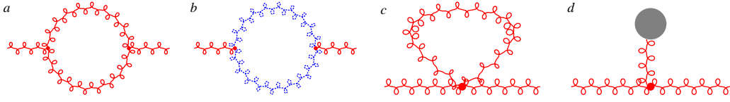
Figure 2: The corrections to the Planck mass is obtained by combining corrections to the graviton propagator (we show the relative Feynman diagrams. Diagram b contains a ghost loop) with corrections to the graviton/matter vertex and with corrections to the matter propagator.
