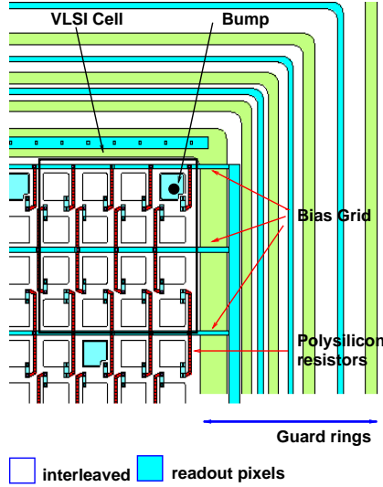
Figure 6: Layout of the proposed detector, corresponding to a 50 μm pitch in both dimensions; the other structures differ by the pitch only
