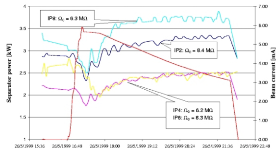
Figure 2: Cryogenic power load vs. beam at 96GeV
