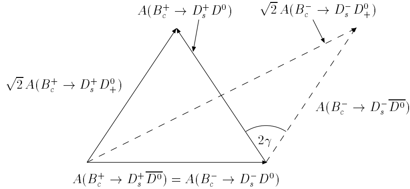
Figure 19. The extraction of \gamma from B_c^\pm \rightarrow D_s^\pm \{D^0, \overline{D^0}, D_+^0\} decays.
