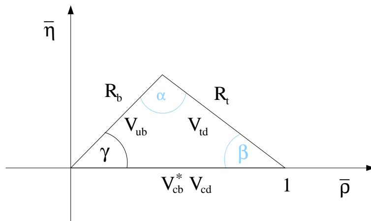
Figure 17. Unitarity triangle in the complex (\bar{\varrho}, \bar{\eta}) plane.
