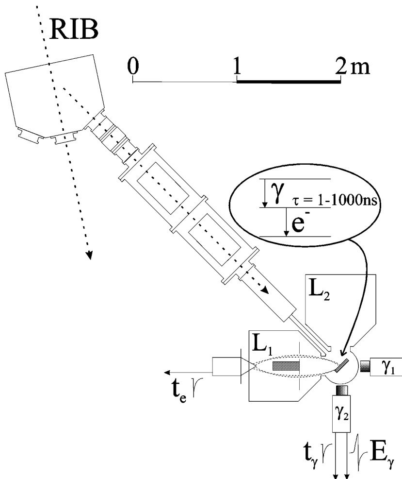
Figure 4. General view of the \gamma - e^- PAC spectrometer mounted on-line with the ISOLDE beam line [18]. Legend: RIB = radioactive ion beams; L_1, L_2 = electron magnetic lens 1 and lens 2; t_e, t_\gamma = anode signals used for time analysis from the electron and gamma photomultipliers, respectively; E_\gamma = dynode signal used for \gamma -ray energy discrimination.
