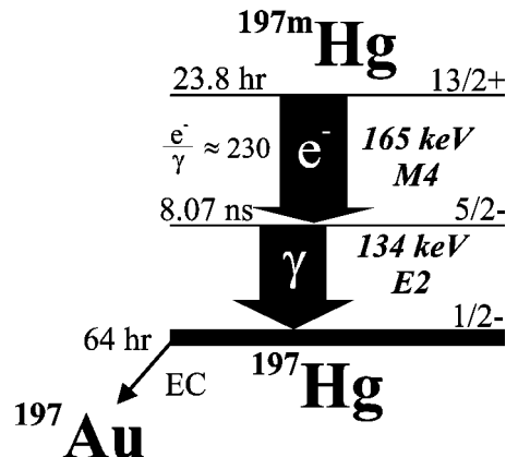
Figure 2. Schematic representation of the decay of ^{197m}\text{Hg} .
