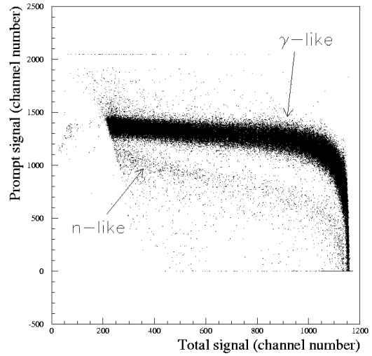
Fig. 5. Second pulse shape discrimination (PSD2) for the N1 detector and the carbon target. Prompt signal amplitude vs. total signal amplitude (different binning).
