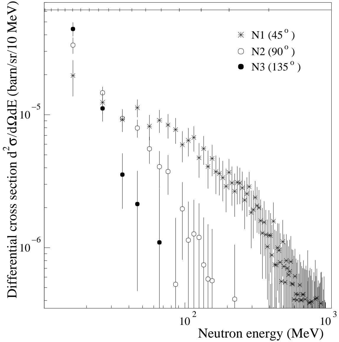
Fig. 8. Neutron energy spectrum for the carbon target, including all the corrections. The spacing between two ticker marks on the upper horizontal line gives the energy resolution (FWHM) at the corresponding energy, derived from the time resolution, for the detector N1.
