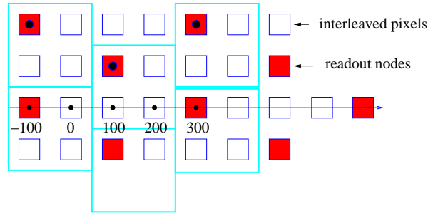
FIGURE 1. A sketch of the tested structure, with 100 \mu m implant pitch and 200 \mu m read-out pitch. The horizontal line identifies the scan direction and defines the coordinate system. The frames define the footprint of an hypothetical VLSI cell.
