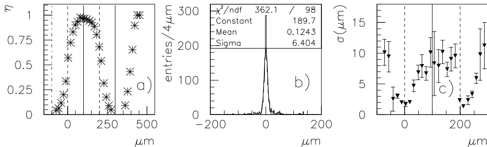
FIGURE 2. The charge sharing among neighbouring read-out pixels, measured by \eta = \frac{PH_i}{PH_{tot}} during the detector scan (a). The average resolution and the achieved resolution vs. the spot position are shown in b) and c). The vertical lines identify the centre of the pixels; the full line identify the reference pixel for the \eta calculation
