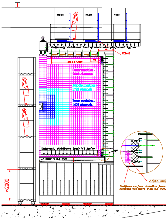
Figure 8: Front view of one half of the electromagnetic calorimeter.
