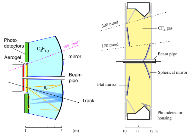
Figure 4: Layout of the RICH1 and RICH2 detectors. The production of two rings in the photo detectors is illustrated for RICH1.
