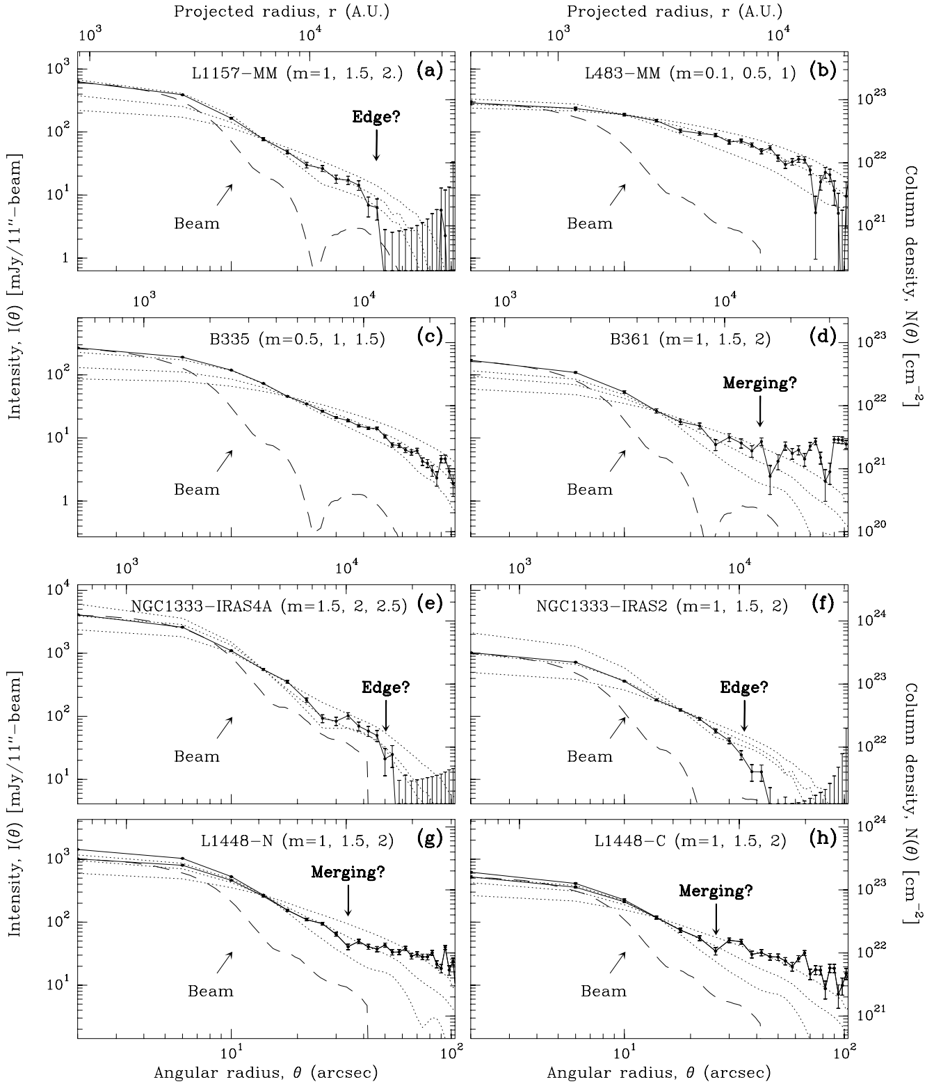
Fig. 4. Same as Fig. 3 for 4 isolated globules (a-d) and 4 Perseus protostars (e-h). See complementary Fig. 12. Column density estimates assume \kappa_{1.3\text{mm}} = 0.01\text{cm}^2\text{g}^{-1} and T_{\text{dust}} = 20\text{K} . In g-h, two source profiles are shown, before (upper solid curve) and after (lower solid curve) subtraction of the disk component observed by the IRAM PdBI interferometer at 1.4 mm (Motte et al. 2001).
