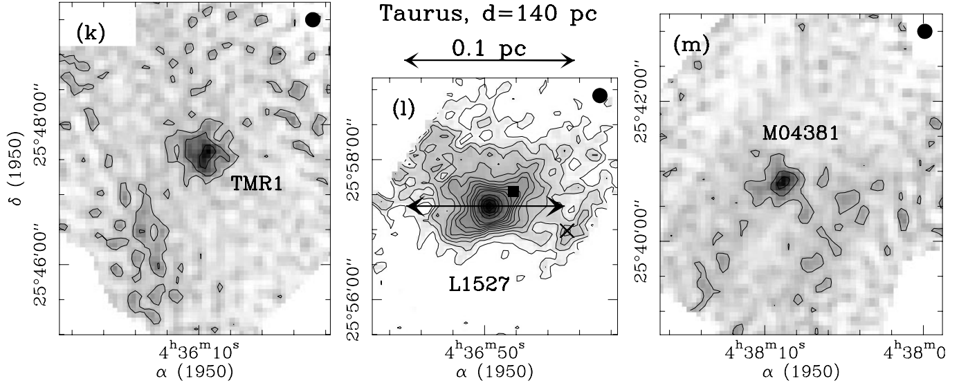
Fig. 1. (cont'd) Contour levels and rms noise at map center are: k 40, 80, 120 mJy/beam, 1\sigma \simeq 11 mJy/beam; l 12 to 120 by 12 mJy/beam and 180 to 420 by 60 mJy/beam, 1\sigma \simeq 3.5 mJy/beam; m 25, 50, 75 mJy/beam, 1\sigma \simeq 7 mJy/beam. The outflow axis and proposed companion of L1527 are marked with arrows and a filled square marker in l (cf. MacLeod et al. 1994 and Fuller, Ladd & Hodapp 1996, respectively).
