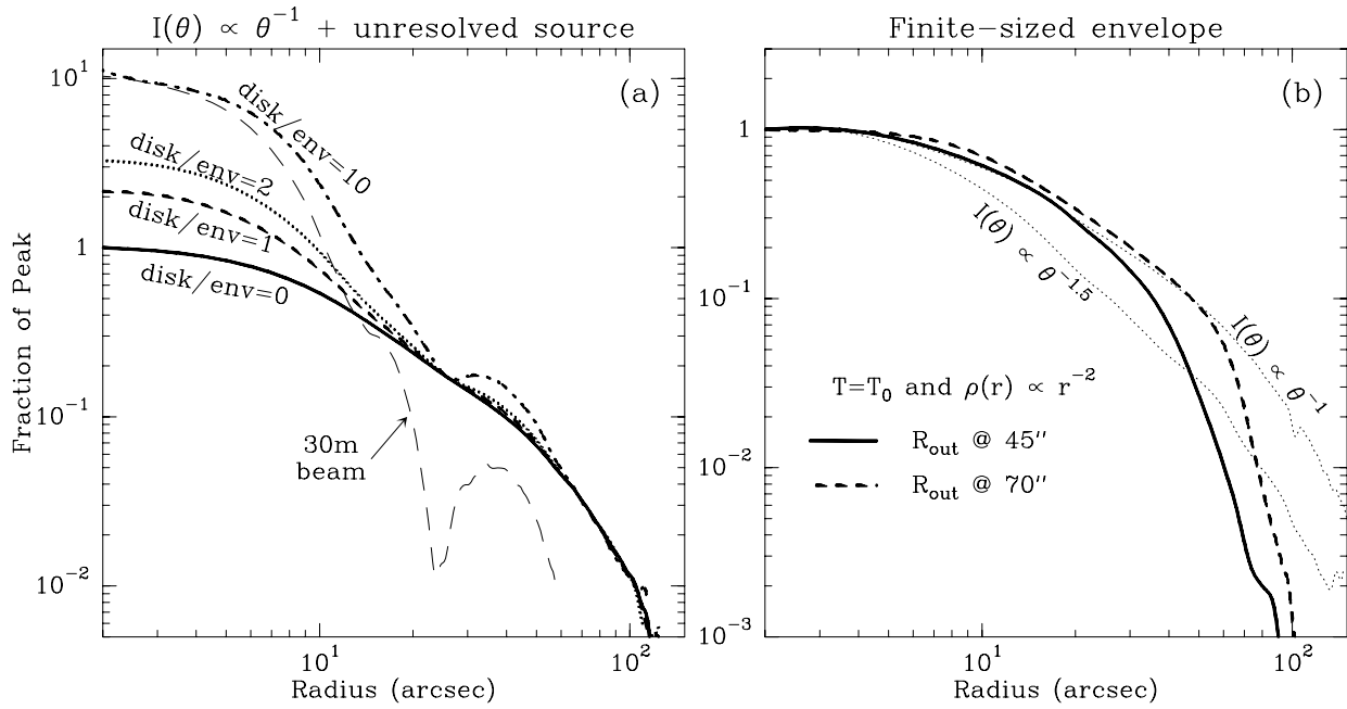
Fig. 8. a Grid of simulated profiles corresponding to a I(\theta) \propto \theta^{-1} input envelope model including an unresolved central source (or disk) characterized by S_{\text{disk}}/S_{\text{env}}^{\text{peak}} = 0, 1, 2 and 10. b Simulated profiles corresponding to finite-sized isothermal envelope models with \rho(r) \propto r^{-2} inside an outer radius corresponding to \theta_{\text{out}} = 45'' and 70'' .
