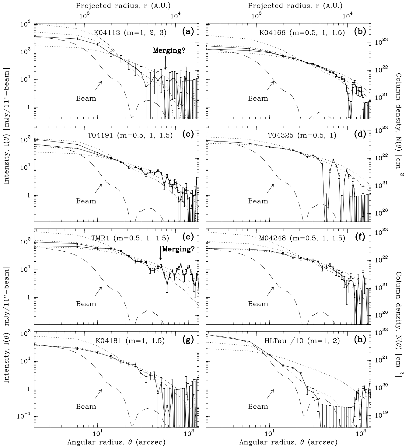
Fig. 11. Complement to Fig. 3. Radial intensity profiles of the environment of 12 Taurus embedded YSOs (a-l) and 4 starless cores (m-p). Column density estimates assuming \kappa_{1.3\text{mm}} = 0.01 \text{ cm}^2 \text{ g}^{-1} and T_{\text{dust}} = 15 \text{ K} are shown on the right axis of each profile (in m-p: \kappa_{1.3\text{mm}} = 0.005 \text{ cm}^2 \text{ g}^{-1} and T_{\text{dust}} = 10 \text{ K} ). The observed profiles (solid curves) are compared with simulated model profiles (dotted curves) and with the 30 m beam (dashed curve). In b-c, e and i, two source profiles are shown, before (upper solid curve) and after (lower solid curve) subtraction of the disk component observed by the IRAM Plateau de Bure interferometer at 1.4 mm (Motte et al. 2001); the latter should correspond to the profile of the envelope alone . The input models are all circularly symmetric with infinite power-law profiles, I(\theta) \propto \theta^{-m} . Unlike YSO envelope profiles, the profiles of starless cores (in m-p) are not consistent with single power-law models.
