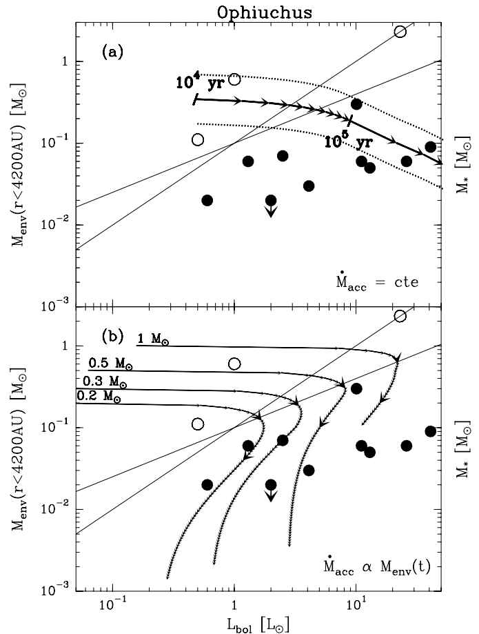
Fig. 6. Same as Fig. 5 for the embedded YSOs of the \rho Ophiuchi main cloud (adapted from AM94). In this case, M_{\text{env}}^{4200\text{AU}} is equivalent to the total envelope mass M_{\text{env}} . Note that, in contrast to the Taurus diagram, there is a gap between Class 0 and Class I objects here.
