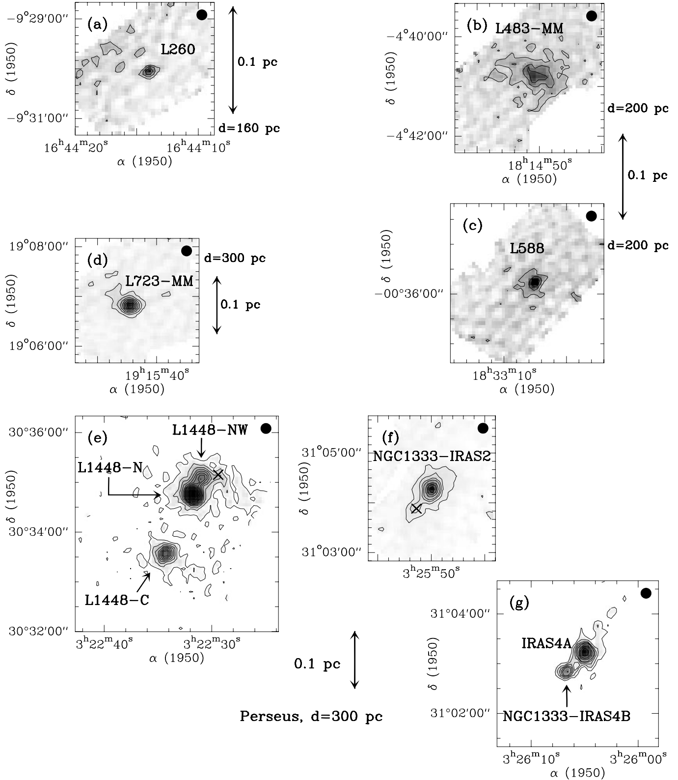
Fig. 10. Complement to Fig. 2. On-the-fly 1.3 mm continuum maps of several isolated globules (a–d) and Perseus protostars (e–g) (all smoothed to a 13'' effective beam). Starless fragments are marked by cross symbols. Contour levels and rms noise at map center are: a 40 to 160 by 40 mJy/beam, 1\sigma \simeq 11 mJy/beam; b 90, 180, 270 mJy/beam, 1\sigma \simeq 26 mJy/beam; c 75, 150, 225 mJy/beam, 1\sigma \simeq 22 mJy/beam; d 35 to 245 by 35 mJy/beam, 1\sigma \simeq 9.5 mJy/beam; e 75 to 600 by 75 mJy/beam and 700 to 1500 by 100 mJy/beam, 1\sigma \simeq 22 mJy/beam; f 75 to 300 by 75 mJy/beam and 450 600 by 750 mJy/beam, 1\sigma \simeq 21 mJy/beam; g 0.2 to 1 by 0.2 Jy/beam and 1.5, 2, 3, 4 Jy/beam, 1\sigma \simeq 55 mJy/beam.
