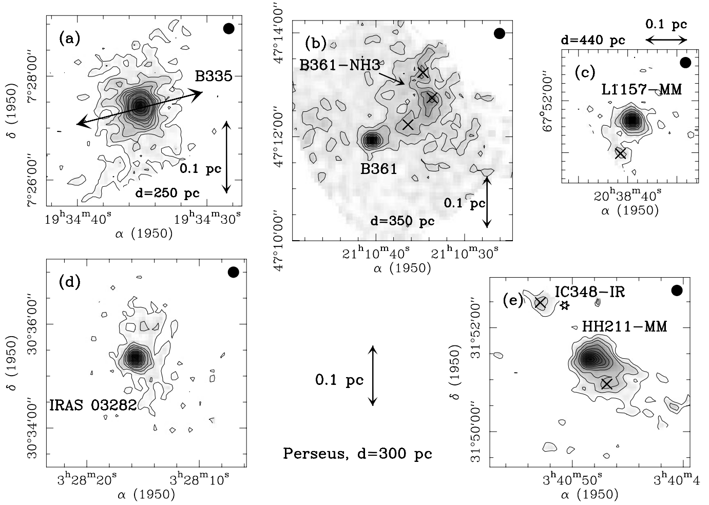
Fig. 2. Same as Fig. 1 for several isolated IRAS globules (a–c) and Perseus protostars (d–e). See complementary Fig. 10. Contour levels and rms noise at map center are: a 12 to 96 by 12 mJy/beam and 150 to 300 by 50 mJy/beam, 1\sigma \simeq 3.5 mJy/beam; b 25 to 175 by 25 mJy/beam, 1\sigma \simeq 7.5 mJy/beam; c 40 to 120 by 40 mJy/beam and 200 to 600 by 80 mJy/beam, 1\sigma \simeq 11 mJy/beam; d 25 to 100 by 25 mJy/beam and 150 to 450 by 50 mJy/beam, 1\sigma \simeq 7.5 mJy/beam; e 30, 60, 90 mJy/beam and 150 to 500 by 50 mJy/beam, 1\sigma \simeq 8.5 mJy/beam. The axis of the B335 outflow is indicated by arrows in a.
