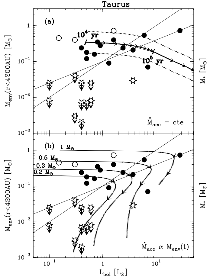
Fig. 5. M_{\text{env}}^{4200\text{AU}} vs. L_{\text{bol}} diagram in Taurus. Bona-fide protostars are shown as (open and filled) circles (for Class 0 and Class I objects, respectively), while peculiar Class I sources are denoted by open star-like markers. The solid straight lines are two M_{\star} - L_{\text{bol}} relations marking the conceptual border zone between the Class 0 stage ( M_{\text{env}}^{4200\text{AU}} > M_{\star} ) and the Class I stage ( M_{\text{env}}^{4200\text{AU}} < M_{\star} ): M_{\star} \propto L_{\text{bol}} (cf. AWB93 and AM94) and M_{\star} \propto L_{\text{bol}}^{0.6} as suggested by the time-dependent accretion scenario of the text (see also AWB2000). Two distinct sets of evolutionary tracks (solid curves) are shown, based on: a A constant accretion rate, \dot{M}_{\text{acc}} \approx 2 \times 10^{-6} M_{\odot} \text{ yr}^{-1} , as in the standard model. Arrows mark time steps from t = 10^4 yr to t = 4 \times 10^5 yr. (The dotted curves illustrate the magnitude of the observational uncertainties on M_{\text{env}}^{4200\text{AU}} .) b A time-dependent accretion rate, \dot{M}_{\text{acc}} \propto M_{\text{env}}(t) , as described in the text. Small arrows are plotted on the tracks every 10^4 yr, big arrows when 50% and 90% of the initial core mass has been accreted.
