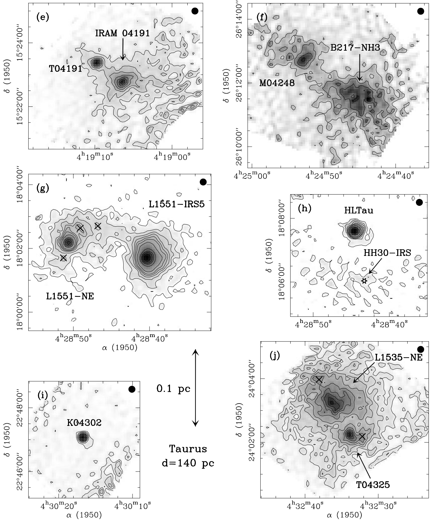
Fig. 1. (cont'd) Contour levels and rms noise at map center are: e 17 to 136 by 17 mJy/beam, 1\sigma \approx 5 mJy/beam; f 17 to 68 by 17 mJy/beam, 1\sigma \approx 5 mJy/beam; g 25 to 150 by 25 mJy/beam, then 200 to 800 by 200 mJy/beam and 1.2, 1.6 Jy/beam, 1\sigma \approx 6 to 9 mJy/beam; h 40 to 200 by 40 mJy/beam and then 300, 600, 900 mJy/beam, 1\sigma \approx 12 mJy/beam; i 17 to 187 by 17 mJy/beam, 1\sigma \approx 5 mJy/beam; j 15 to 135 by 15 mJy/beam, 1\sigma \approx 4.5 mJy/beam.
