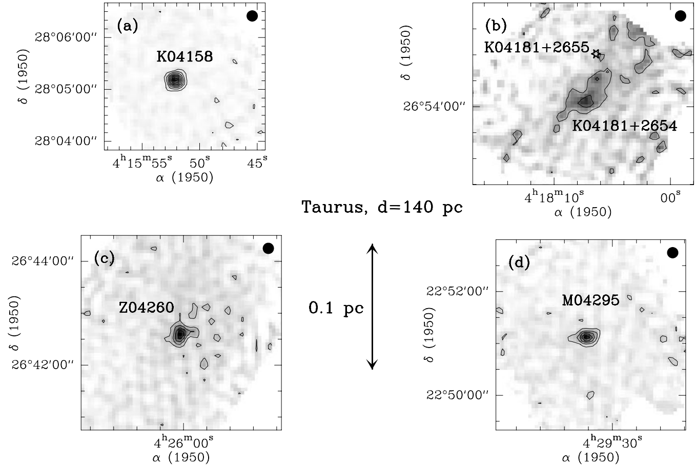
Fig. 9. Complement to Fig. 1. On-the-fly 1.3 mm continuum maps of Taurus embedded YSOs smoothed to a 13'' angular resolution. The positions of YSOs with weak emission are marked by star symbols. Contour levels and rms noise at map center are: a 17 to 136 by 17 mJy/beam, 1\sigma \simeq 5 mJy/beam; b 20 to 40 mJy/beam, 1\sigma \simeq 6 mJy/beam; c 25 to 100 by 25 mJy/beam, 1\sigma \simeq 6.5 mJy/beam; d 20 to 100 by 20 mJy/beam, 1\sigma \simeq 6.5 mJy/beam.
