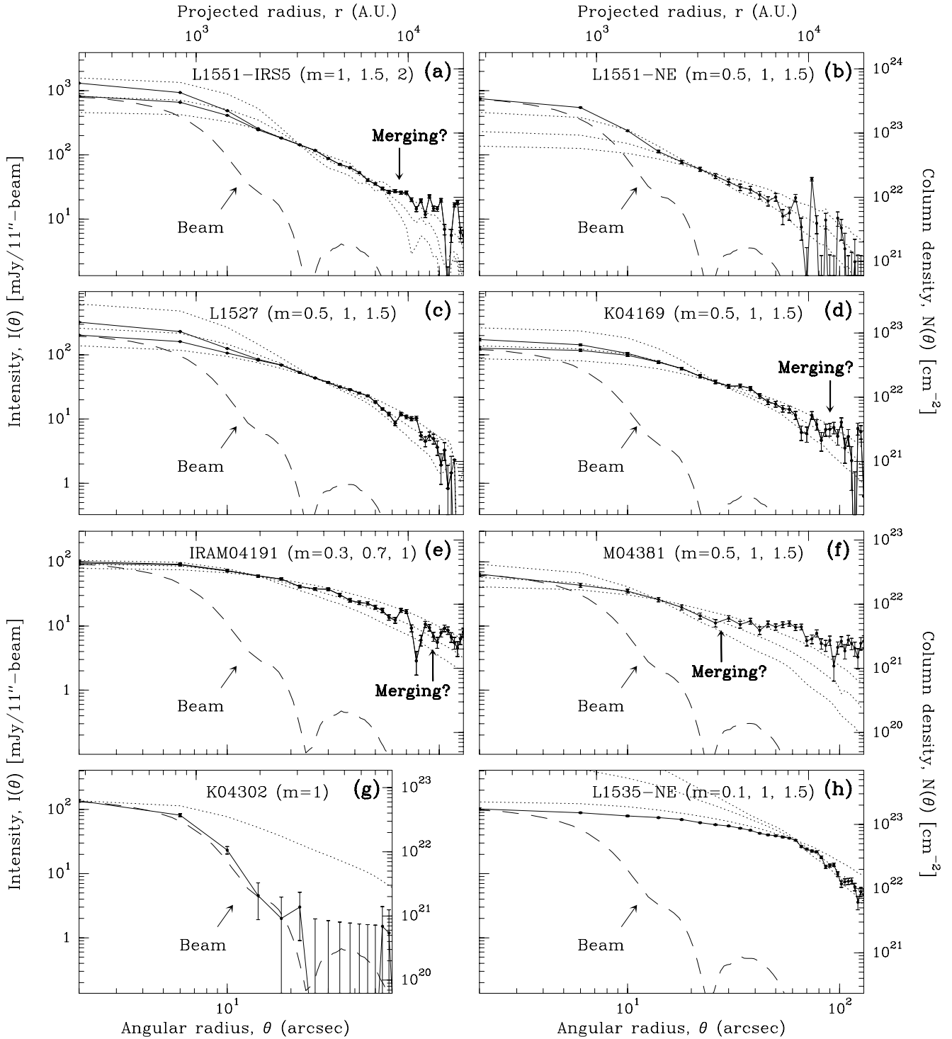
Fig. 3. Radial intensity profiles of the environment of 7 embedded YSOs (a-g) and 1 starless core (h). See complementary Fig. 11. Column density estimates assuming \kappa_{1.3\text{mm}} = 0.01 \text{ cm}^2 \text{ g}^{-1} and T_{\text{dust}} = 15 \text{ K} are shown on the right axis of each profile (in h: \kappa_{1.3\text{mm}} = 0.005 \text{ cm}^2 \text{ g}^{-1} and T_{\text{dust}} = 10 \text{ K} ). The observed profiles (solid curves) are compared with simulated model profiles (dotted curves) and with the 30 m beam (dashed curve). In a and c-e, two source profiles are shown, before (upper solid curve) and after (lower solid curve) subtraction of the disk component observed by the IRAM Plateau de Bure interferometer at 1.4 mm (Motte et al. 2001); the latter should correspond to the profile of the envelope alone . The input models are all circularly symmetric with infinite power-law profiles, I(\theta) \propto \theta^{-m} (see Appendix). Unlike YSO envelope profiles, the profile of the starless core L1535-NE (in h) is not consistent with a single power-law model.
