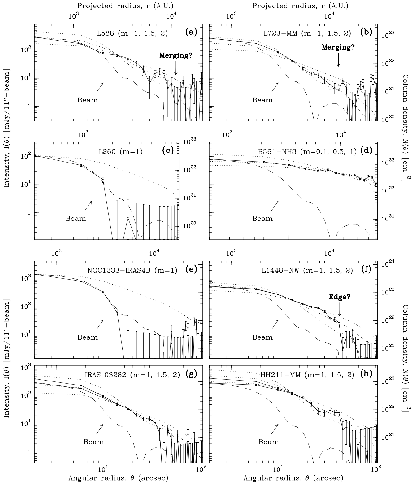
Fig. 12. Complement to Fig. 4. Radial intensity profiles of the environment of 3 isolated IRAS globules (a-c), 4 Perseus protostars (e-h), and 1 starless core (d). Column density estimates assume \kappa_{1.3\text{mm}} = 0.01 \text{ cm}^2 \text{ g}^{-1} and T_{\text{dust}} = 20 \text{ K} . In f-h, two source profiles are shown, before (upper solid curve) and after (lower solid curve) subtraction of the disk component observed by the IRAM PdBI interferometer at 1.4 mm (Motte et al. 2001). Unlike YSO envelope profiles, the profile of the starless core B361-NH3 (in d) is not consistent with a single power-law model.
