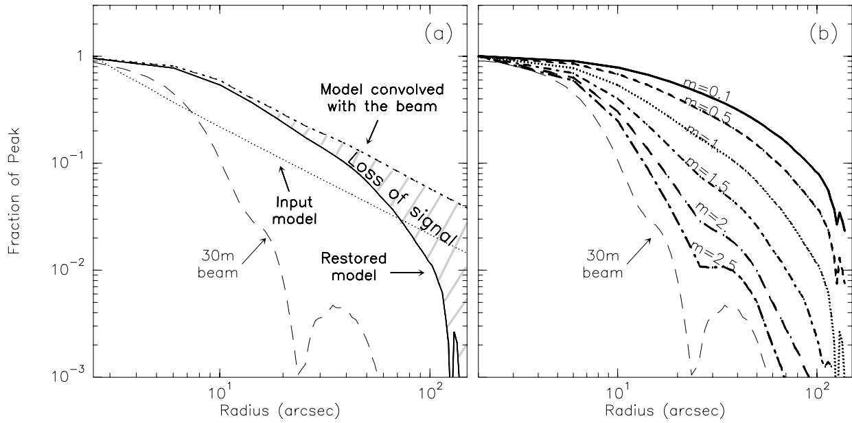
Fig. 7. a Effect of the dual-beam observing technique on the observed radial intensity profiles. The dash-dotted curve represents an input model with I(\theta) \propto \theta^{-1} (cf. dotted line) after convolution with the beam of the telescope (dashed curve). The solid curve shows the output model profile that results from our simulation of the dual-beam observation and the various data reduction steps. b Grid of simulated profiles for a range of input power-law models, I(\theta) \propto \theta^{-m} , with m = 0.1 to 2.5.
