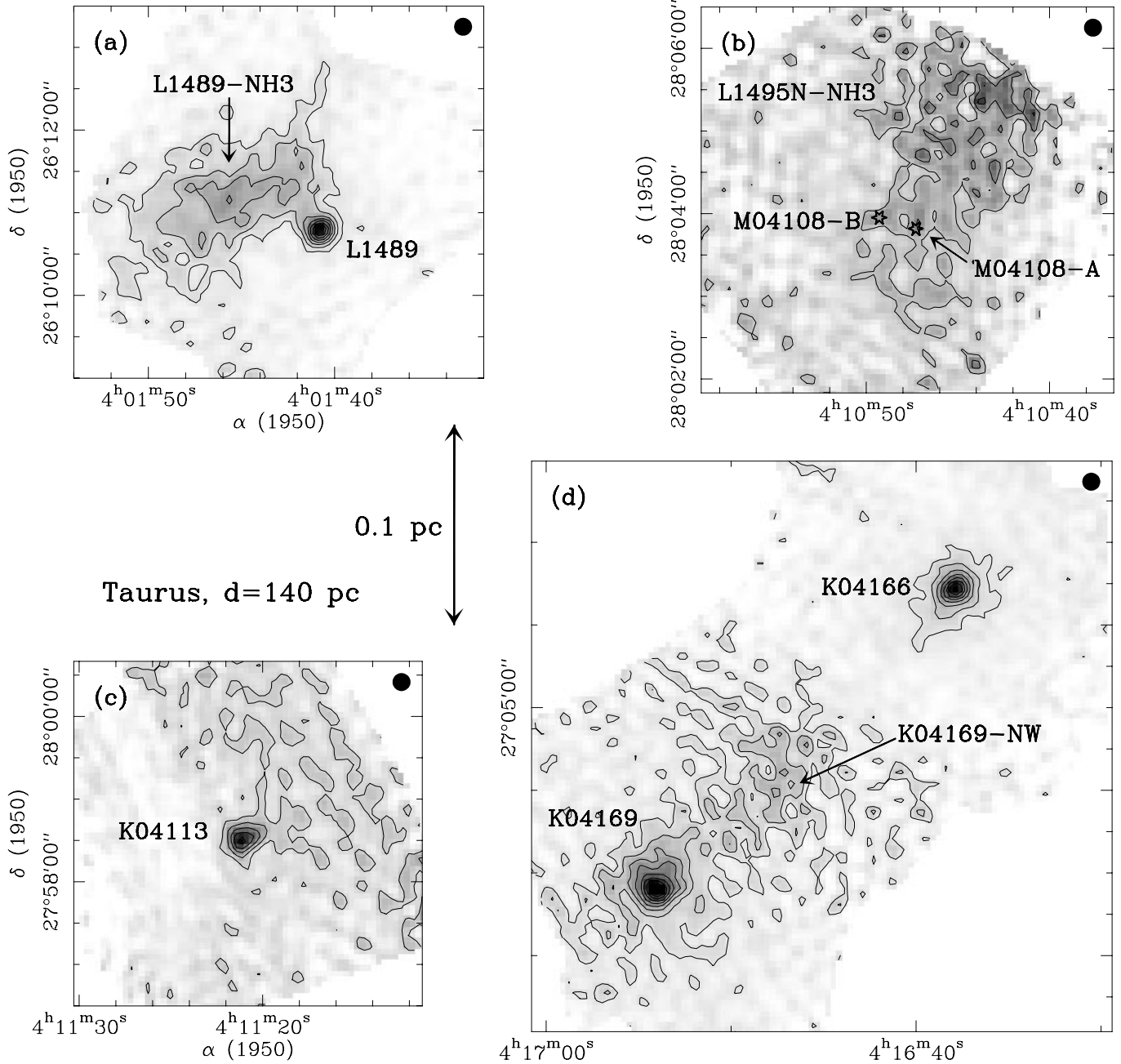
Fig. 1. Selection of on-the-fly 1.3 mm continuum maps obtained toward Taurus embedded YSOs (all smoothed to a 13'' effective beam). See complementary Fig. 9. The positions of YSOs with weak emission and starless fragments are marked by stars and crosses, respectively. Contour levels and rms noise at map center are: a 15 to 120 by 15 mJy/beam, 1\sigma \simeq 4 mJy/beam; b 35, 70, 105 mJy/beam, 1\sigma \simeq 9.5 mJy/beam; c 90 to 450 by 90 mJy/beam, 1\sigma \simeq 27 mJy/beam; d 25 to 200 by 25 mJy/beam, 1\sigma \simeq 6 to 7 mJy/beam.
