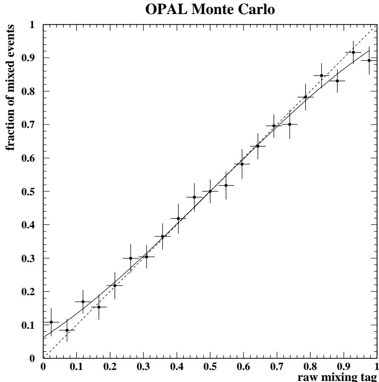
Figure 8: Deviation of mixing tag from a true probability. The points with the error bars show simulated events, the solid line is a fit to these points as described in the text and the dotted line is M = x , representing a true probability requiring no correction. The error bars include systematic errors described in Section 9. Both charge conjugated cases were added to maximize the statistical significance.
