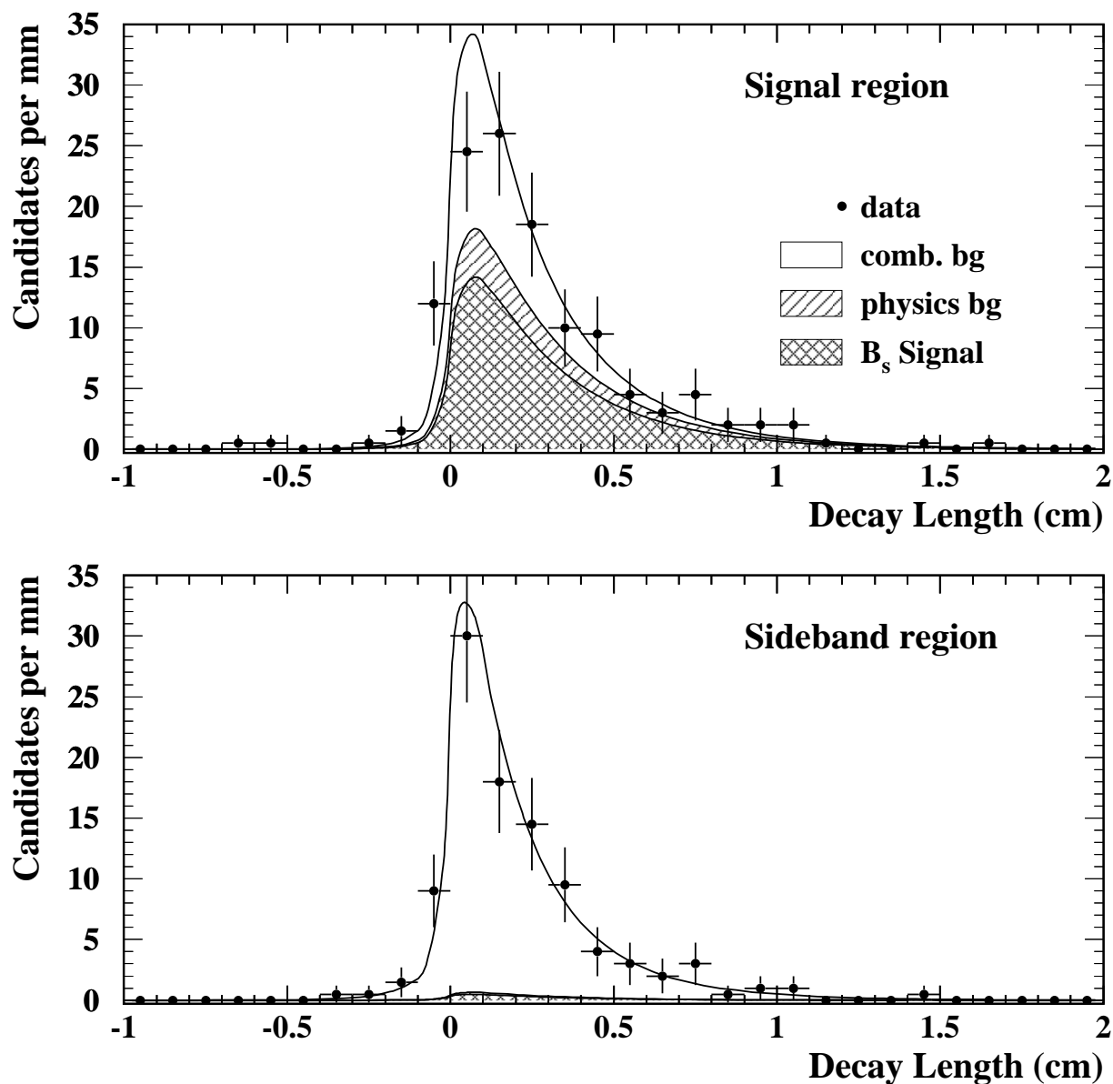
Figure 10: Comparison of expectation from fit results and actual decay length distributions. The fit results are shown by the curves, with individual components shaded, while the decay lengths measured in the data are shown by the error bars. The sideband region was used in the combinatorial background lifetime fit.
