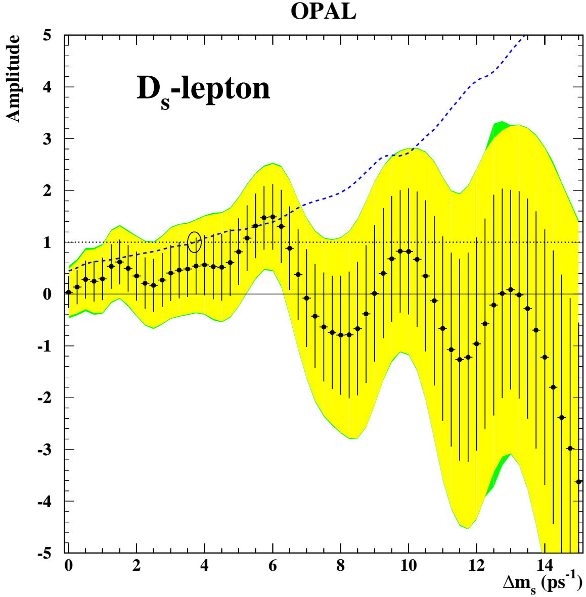
Figure 9: Measured B_s oscillation amplitude as a function of \Delta m_s for this analysis. The error bars represent the 1\sigma statistical uncertainties. The shaded bands show the \pm 1.645\sigma region, with and without including systematic effects. The values of \Delta m_s where the shaded region lies below the \mathcal{A} = 1 line are excluded at the 95% confidence level. The dashed line is 1.645\sigma used to determine the experimental sensitivity, which is indicated by the circle.
