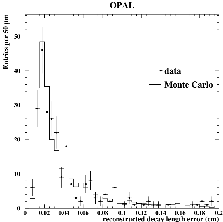
Figure 2: Distribution of reconstructed decay length errors for selected events. The points with the error bars represent the data while the histogram represents the simulated events.
