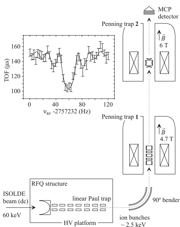
Figure 1: Experimental setup of the ISOLTRAP mass spectrometer. The inset shows the cyclotron resonance curve for ^{33}\text{Ar} . Plotted is the time of flight (TOF) of the ions from the trap to the ion detector as a function of the applied radio frequency. The solid line is a fit of the theoretical line shape [9] to the data points.
