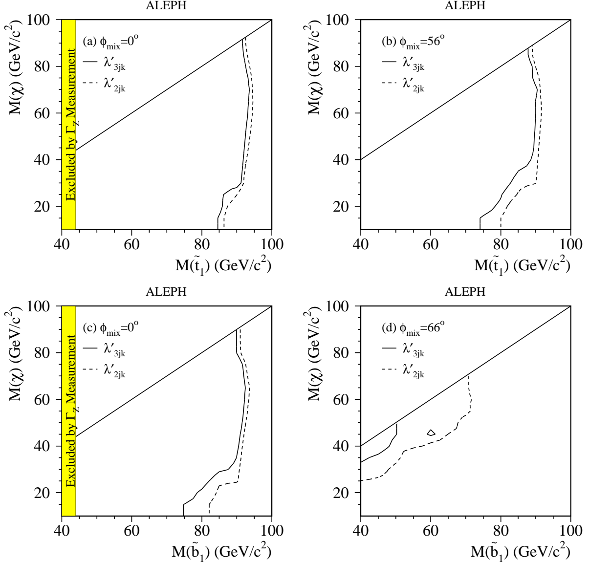
Figure 9: The 95% C.L. limits in the (M_\chi, M_{t_1}) and (M_\chi, M_{b_1}) planes for indirect LQ\bar{D} decays via the \lambda'_{211} and \lambda'_{311} couplings, for no squark mixing ( \phi_{\text{mix}} = 0^\circ ) and for \phi_{\text{mix}} = 56^\circ, 66^\circ for stops and sbottoms, respectively.
