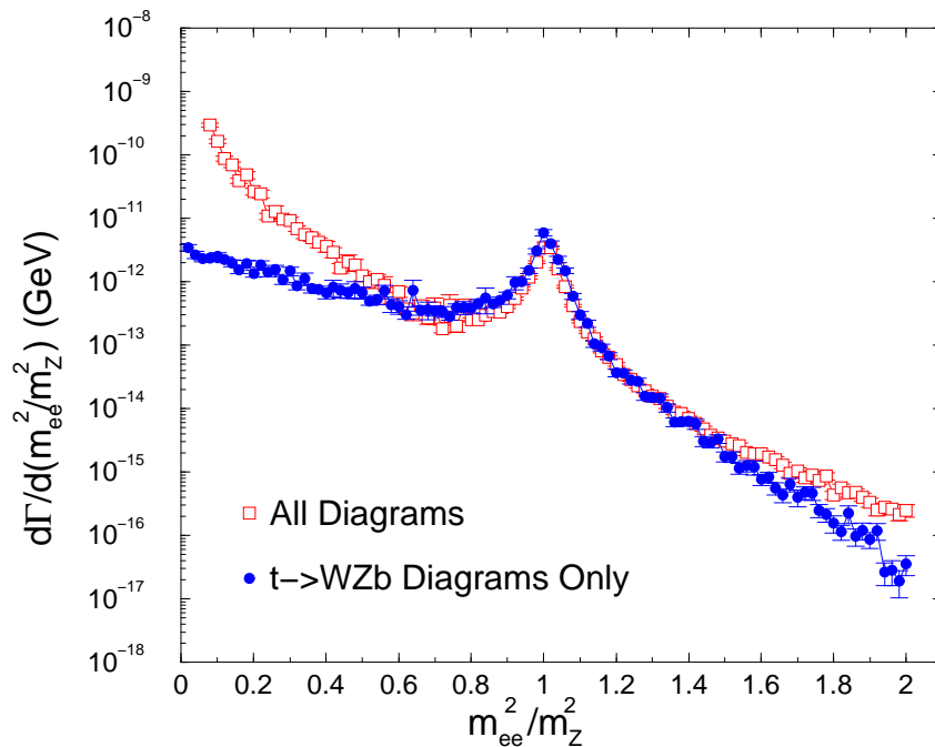
Figure 4: The differential rate d\Gamma/d(m_{ee}^2/m_Z^2) , for the t \rightarrow b\mu\nu_\mu e^+ e^- decay, computed by considering all Feynman diagrams contributing to the process or only the three relevant diagrams which proceeds through the initial t \rightarrow WZb decay. The top quark mass is fixed to m_t = 175 GeV.
