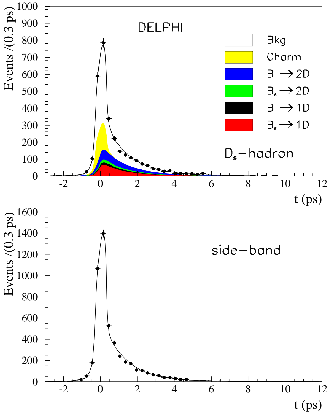
Figure 9: D_s^\pm h^\mp analysis. Upper plot: Proper time distribution for events in the signal mass region. The points show the data and the shaded regions correspond to the different contributions to the selected events. The curve shows the result of the fit described in the text. Lower plot: the same as the upper plot but for events situated in the D_s mass side-band.
