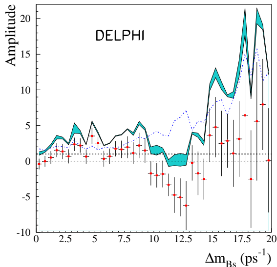
Figure 5: Exclusive B_s^0 analysis: variation of the oscillation amplitude A as a function of \Delta m_{B_s^0} . The lower continuous line corresponds to A + 1.645 \sigma(A) where \sigma(A) includes statistical uncertainties only, while the shaded area shows the contribution from systematics. The dashed-dotted line corresponds to the sensitivity curve. The lines at A=0 and A=1 are also given. The points with error bars are real data.
