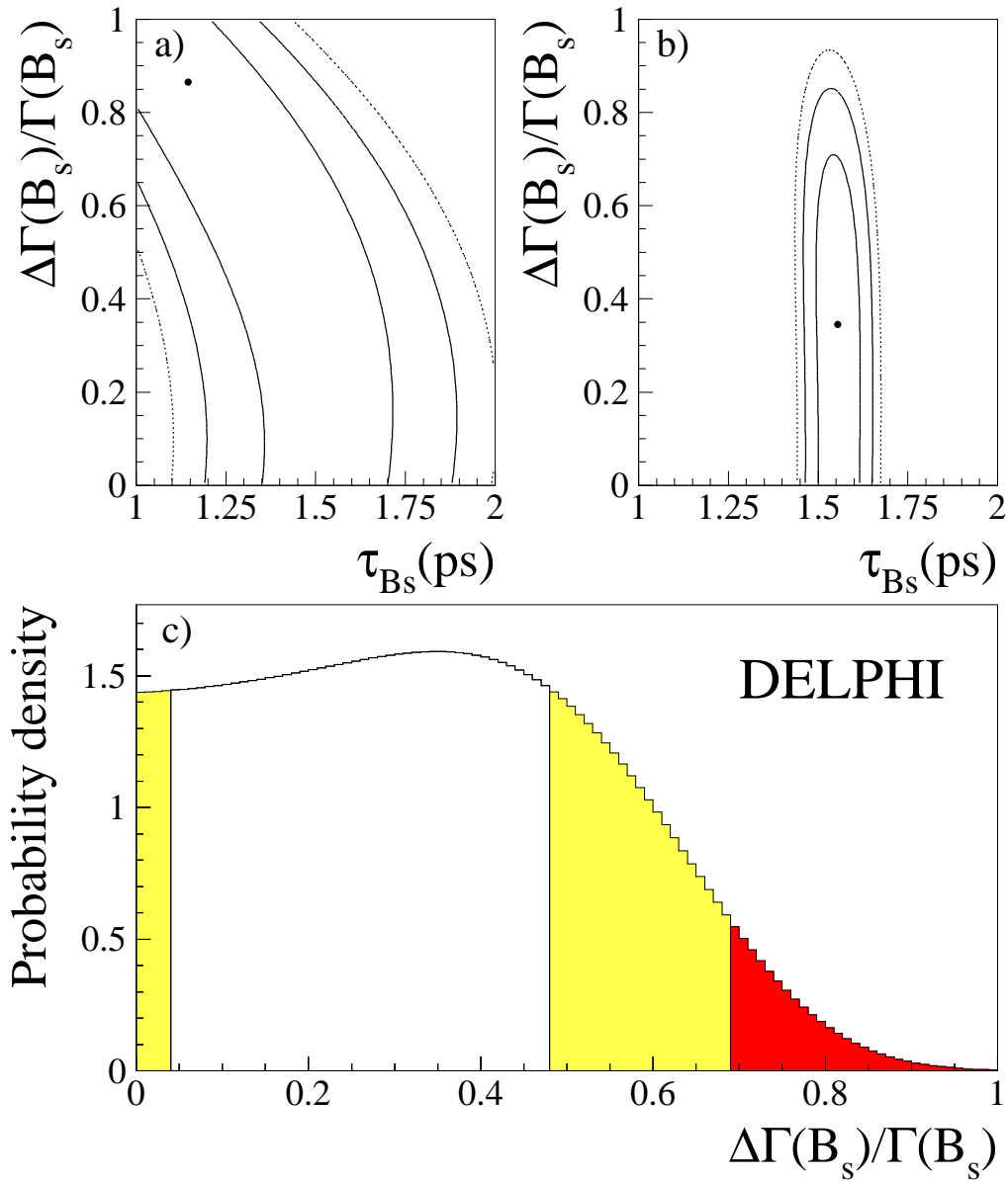
Figure 10: D_s^{\pm} h^{\mp} analysis: 68%, 95%, 99% C.L. contours of the negative log-likelihood in the plane \Delta\Gamma_{B_s^0}/\Gamma_{B_s^0} - \tau_{B_s^0} a) without and b) with \tau_{B_s} = \tau_{B_s^0} constraint. The point indicates the minimum. c) Probability density distribution for \Delta\Gamma_{B_s}/\Gamma_{B_s} ; the two lightly shaded regions at the 68% C.L. and dark one at the 95% C.L. are also shown.
