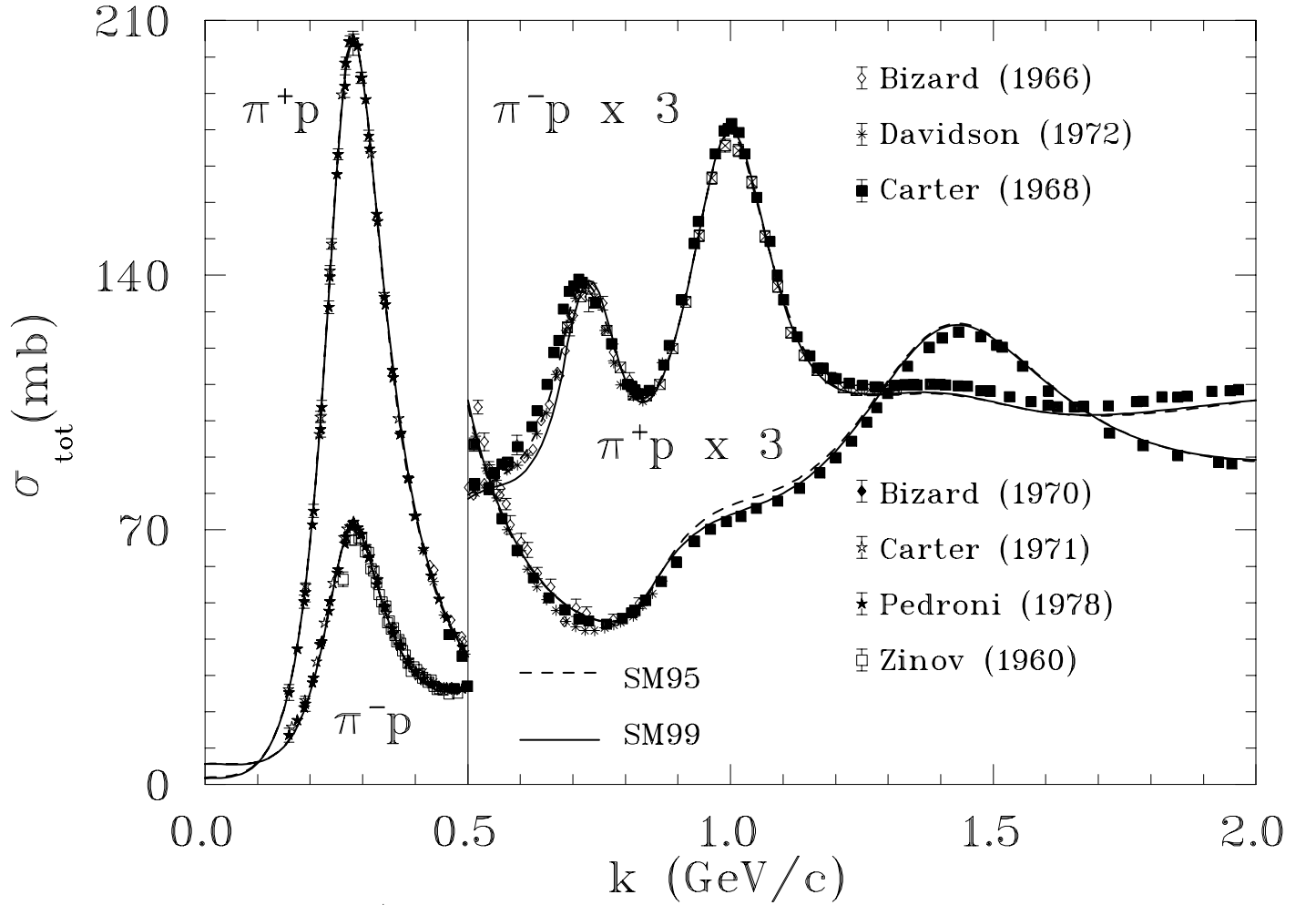
FIG. 2. The experimental total \pi^+p and \pi^-p cross sections below 2 GeV/c [59–65] compared with the SM95 [58] and SM99 [29] PWA hadronic solutions, where Coulomb barrier effects have not been taken into account.
