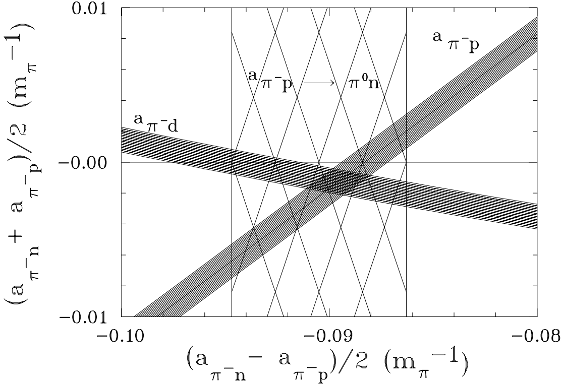
FIG. 1. Graphical determination of the \pi N scattering lengths (a_{\pi-p} + a_{\pi-n})/2 \simeq a^+ and (a_{\pi-p} - a_{\pi-n})/2 \simeq a^- from the constraints imposed by the pionic atom scattering lengths.
