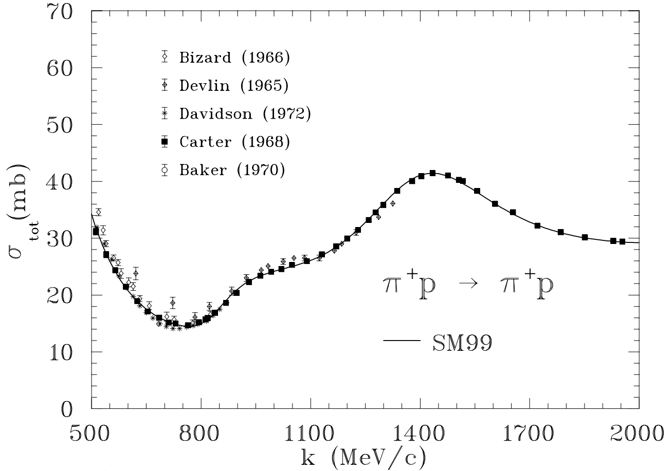
FIG. 5. The \pi^+p experimental total cross sections in the region 0.5 \leq k \leq 2 GeV/c [59–61,69,70] compared to SM99 [29] with Coulomb barrier effects accounted for.
