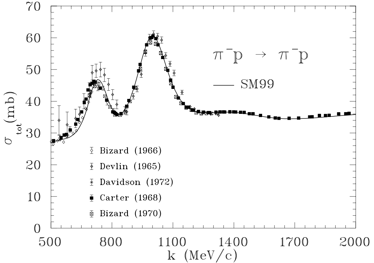
FIG. 4. The \pi^- p experimental total cross sections in the region 0.5 \leq k \leq 2 GeV/c [59–62,69] compared to SM99 [29] with Coulomb barrier effects accounted for.
