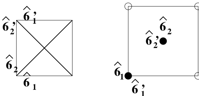
Figure 2: Configuration of \widehat{\text{D6}} -branes in the \Omega'\alpha orientifold of \mathbf{T}^4/\mathbf{Z}_2 , for R_1 = 1 , R_2 > 1 .
