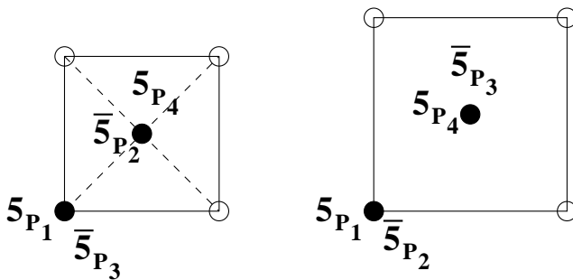
Figure 1: Configuration of D5- and \overline{\text{D5}} -branes in the \Omega'\alpha orientifold of \mathbf{T}^4/\mathbf{Z}_2 , for R_1 = 1 , R_2 > 1 . Discontinuous lines denote strings stretched between D5-branes at P_1 and \overline{\text{D5}} -branes at P_2 , which lead to tachyonic modes for R_1 < 1 .
