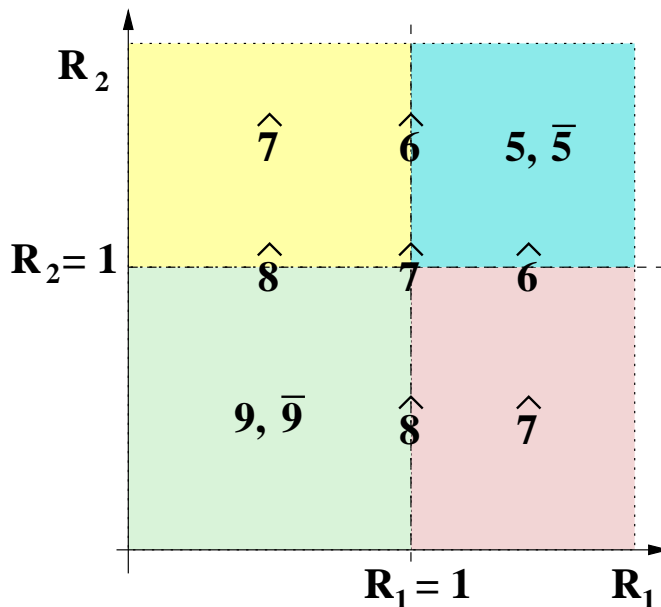
Figure 4: Phase diagram for the \Omega'\alpha orientifold of \mathbf{T}^4/\mathbf{Z}_2 . For large R_1, R_2 the stable configuration corresponds to a set of D5- and \overline{\text{D}}5 -branes at orbifold fixed points. When one of the radii decreases below the critical value R = 1 , brane-antibrane pairs decay into non-BPS \widehat{\text{D}}7 -branes, wrapped in the small two-torus and transverse to the large one. For R_1, R_2 < 1 , the stable configuration contains a set of D9- and \overline{\text{D}}9 -branes. When one or two of the radii are exactly equal to the critical value, there exist marginally tachyon-free configurations. For instance, configurations of non-BPS \widehat{\text{D}}6 -branes partially wrapping a 1-cycle in the first plane, and transverse to the second, for R_1 = 1, R_2 > 1 ; configurations of non-BPS \widehat{\text{D}}8 -branes partially wrapping a 1-cycle in the first plane, and completely wrapped on the second, for R_1 = 1, R_2 < 1 ; and a configuration of non-BPS \widehat{\text{D}}7 -branes wrapping one 1-cycle on each plane for R_1 = 1, R_2 = 1 .
