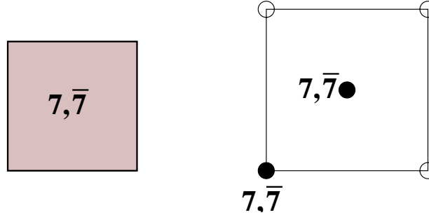
Figure 3: Configuration of D7-\overline{D7} pairs in the \Omega'\alpha orientifold of \mathbf{T}^4/\mathbf{Z}_2 , for R_1 = 1 . The branes wrap the first (shaded) complex plane, and sit at the dot locations in the second.
