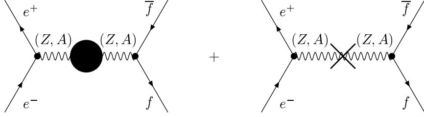
Fig. 15: Process e^+e^- \rightarrow (Z, A) \rightarrow f\bar{f} ; self energies and kinetic counter-terms.
