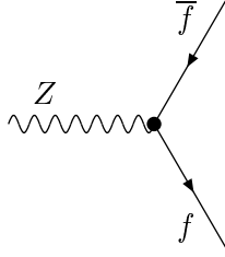
Fig. 9: Process Z \rightarrow f\bar{f} ; Born approximation.
