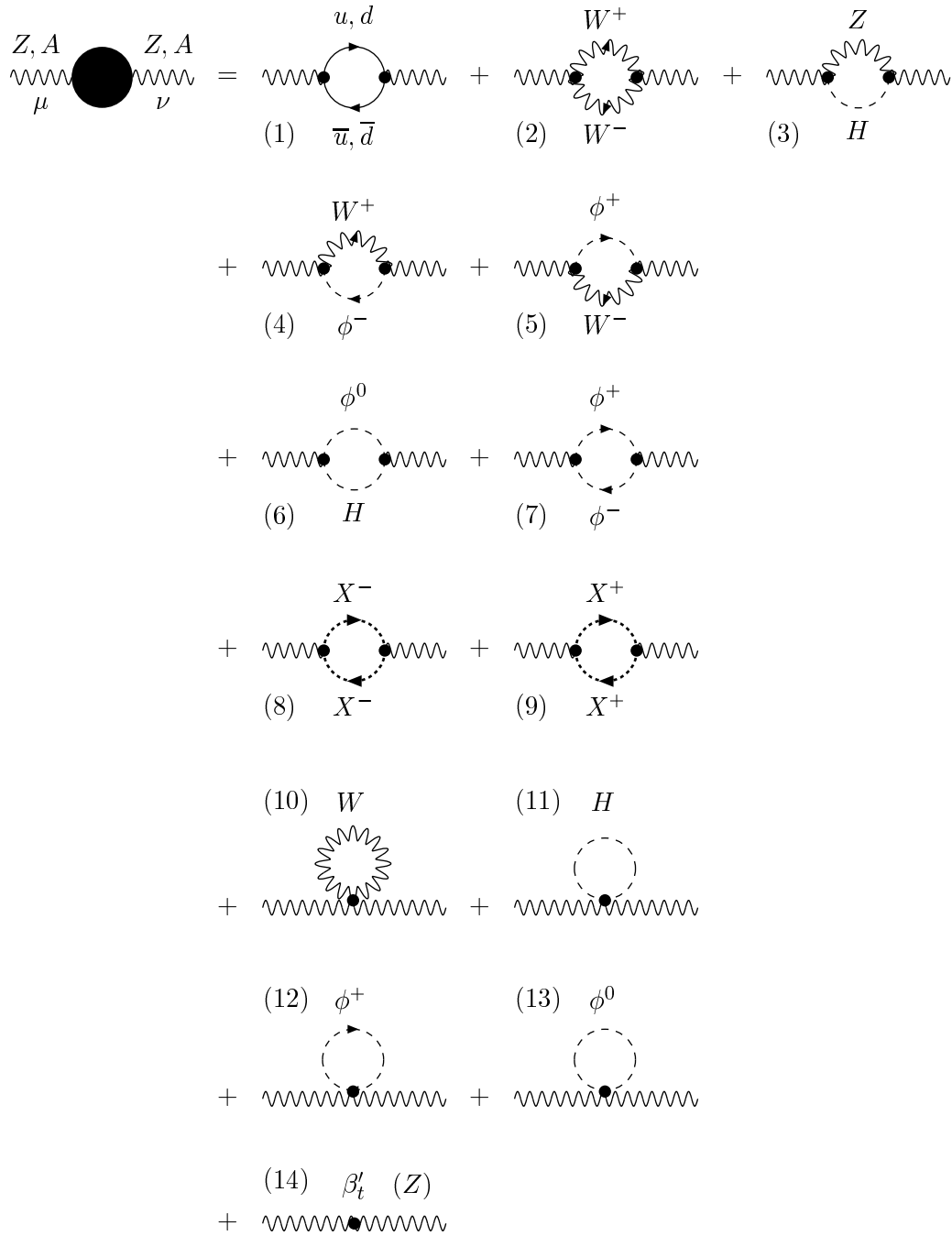
Fig. 5: (Z, A) -boson self-energy; Z - A transition.
