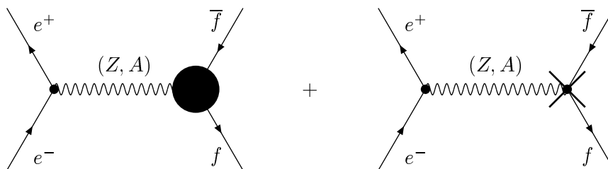
Fig. 13: Process e^+e^- \rightarrow (Z, A) \rightarrow f\bar{f} ; final fermion vertex and its counter-terms.
