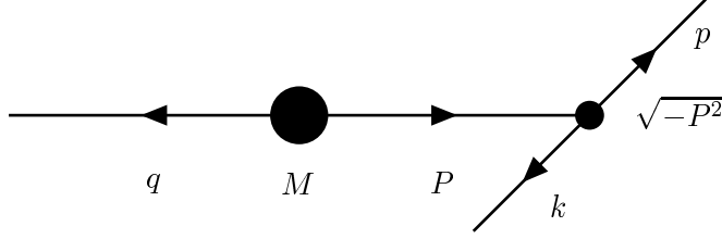
Fig. 4: Kinematical cascade for the 1 \rightarrow 3 decay.
