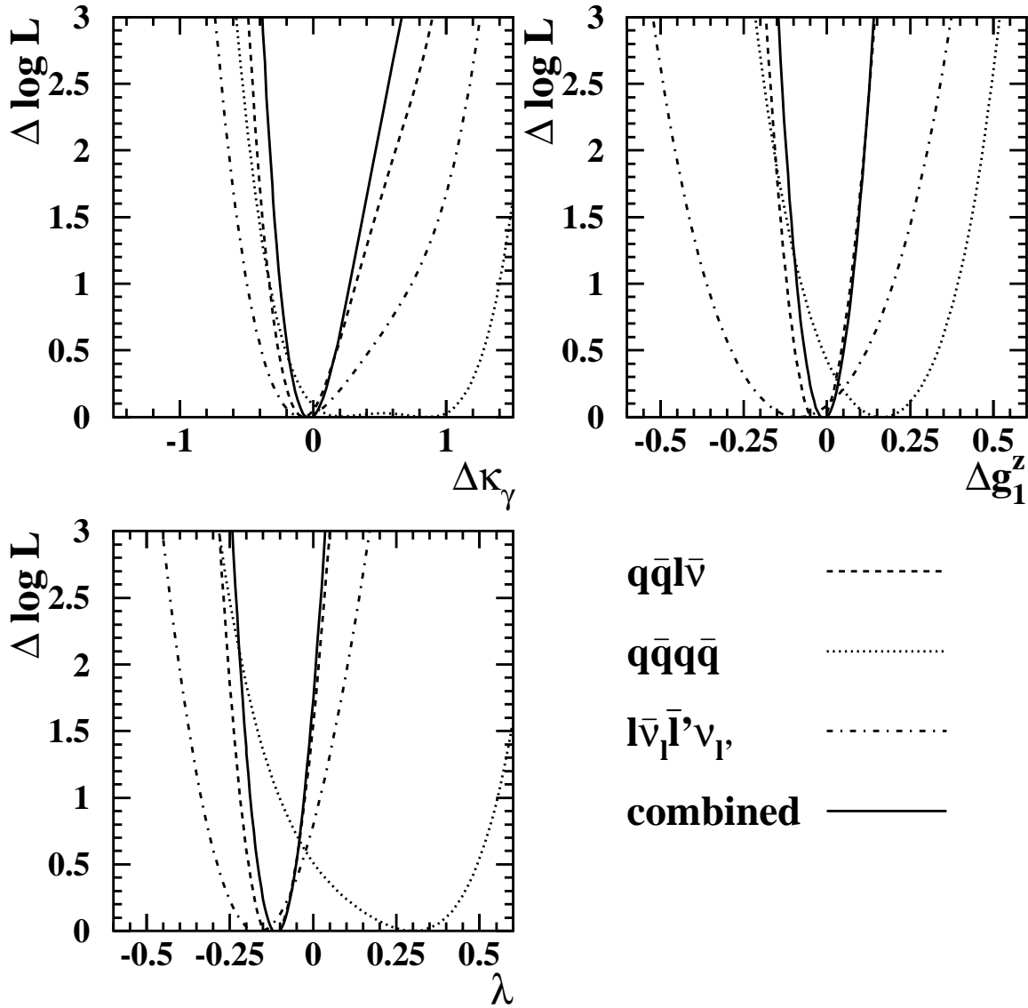
Figure 6: Negative log-likelihood curves obtained from the different final states: q\bar{q}l\bar{\nu}_\ell (dashed lines), q\bar{q}q\bar{q} (dotted lines) and l\bar{\nu}_\ell\ell'\nu_{\ell'} (dash-dotted lines). Each curve is obtained by combining the results from the event shapes and the event rates and setting the other two TGC parameters to their Standard Model values. Systematic errors are included. The solid line is obtained by combining the three final states.
