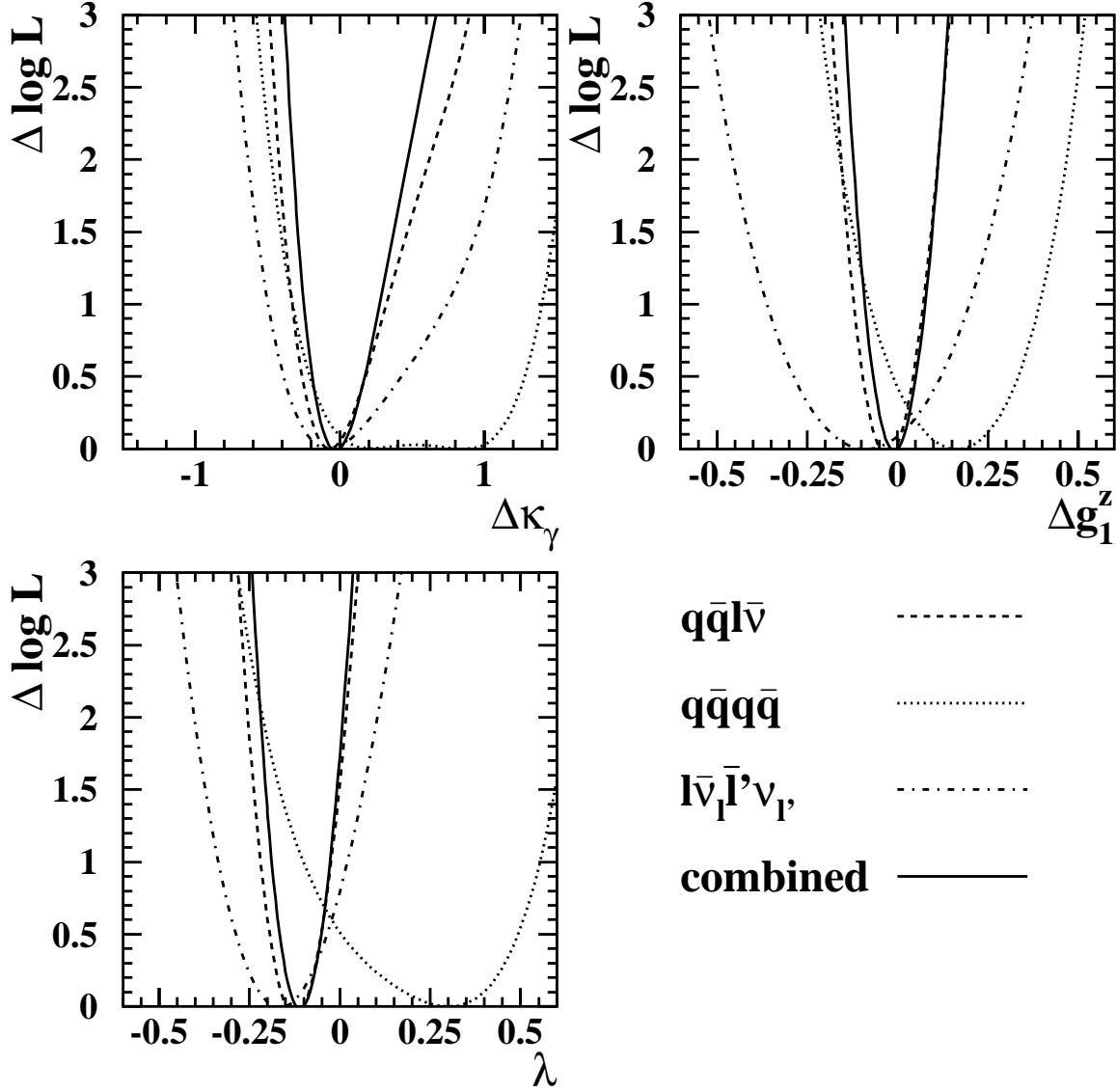
Figure 6: Negative log-likelihood curves obtained from the different final states: q\bar{q}l\bar{\nu}_\ell (dashed lines), q\bar{q}q\bar{q} (dotted lines) and l\bar{\nu}_\ell l' \bar{\nu}_{\ell'} (dash-dotted lines). Each curve is obtained by combining the results from the event shapes and the event rates and setting the other two TGC parameters to their Standard Model values. Systematic errors are included. The solid line is obtained by combining the three final states.
