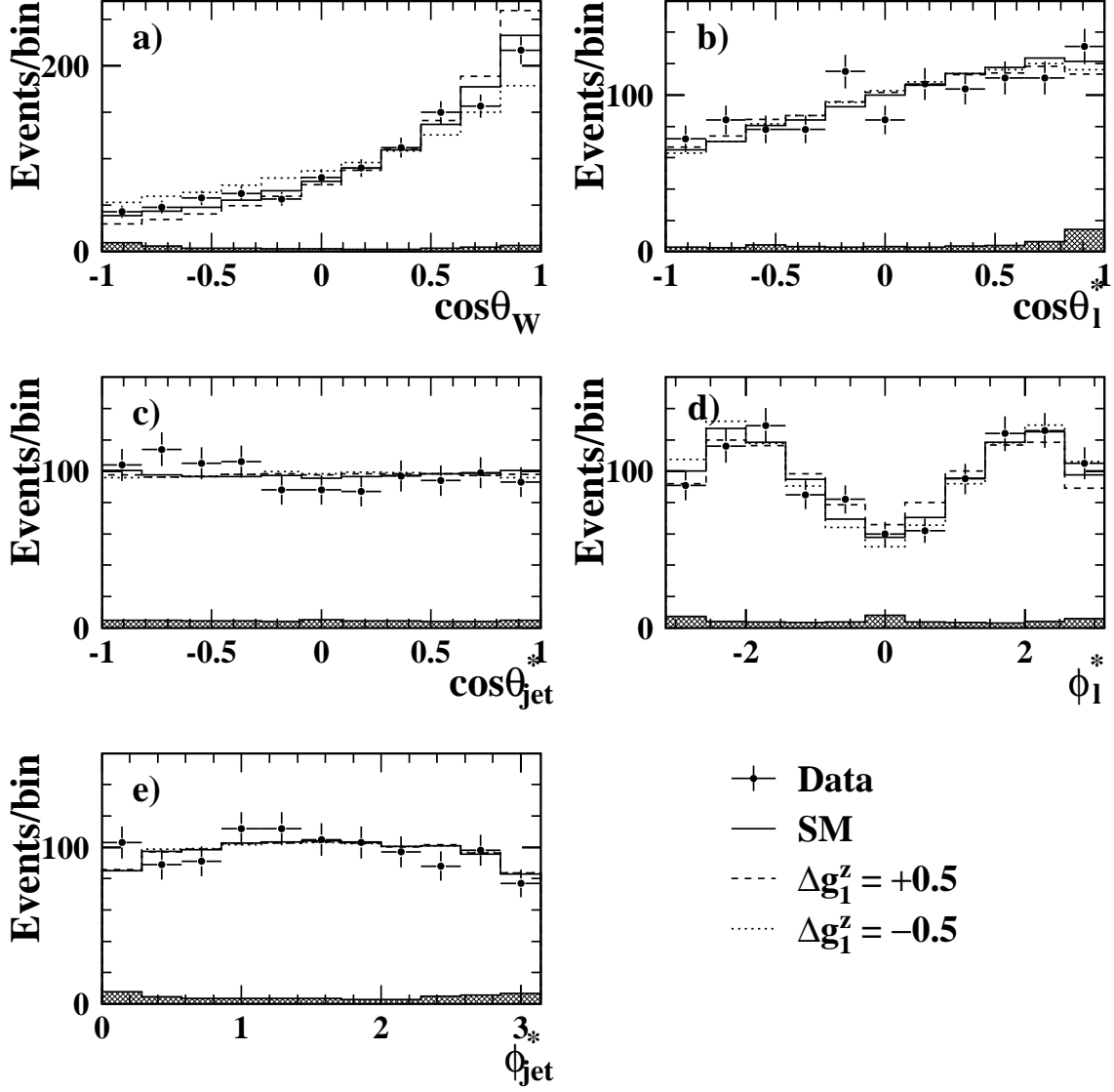
Figure 1: Distributions of the kinematic variables \cos\theta_W , \cos\theta_\ell^* , \cos\theta_{jet}^* , \phi_\ell^* and \phi_{jet}^* , as obtained from the q\bar{q}\ell\nu_\ell events. The solid points represent the data. The histograms show the expectation of the Standard Model and when \Delta g_1^z = \pm 0.5 . The shaded histogram shows the non- q\bar{q}\ell\nu_\ell background. Notes: 1. In the case of W^+ \rightarrow \bar{\ell}\nu decays the value of \phi_\ell^* is shifted by \pi in order to overlay W^+ and W^- distributions in the same plot. 2. The jet with 0 \leq \phi_{jet}^* \leq \pi is chosen as the quark (antiquark) jet from the decay of the W^- ( W^+ ) according to our convention.
