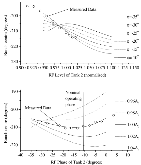
Figure 4. Measured data for the phase position of the bunch at the output of tank 2 as a function of a) the RF amplitude and b) the RF phase. Curves show simulated bunch phase position.
